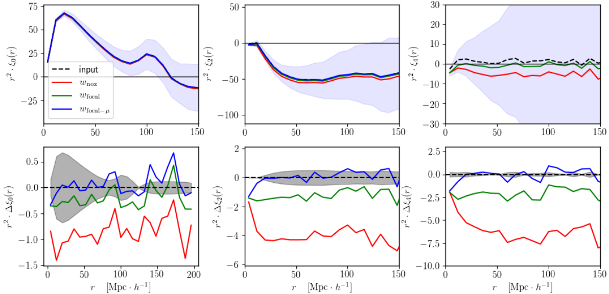
Figure 13. Effect of the different weighting schemes on the correlation function multipole (left: monopole, middle: quadrupole, right: hexadecapole). \mathcal{W}_{\text{noz}} (red curves): upweighting of the nearest neighbour for redshift failures. \mathcal{W}_{\text{focal}} (green curves): weight according to the inverse of the spectroscopic efficiency. \mathcal{W}_{\text{focal}-\mu} (blue curves): same as \mathcal{W}_{\text{focal}} but the \mu > 1 - 1/480 region is removed as described in the text. The light-blue shaded bands on the top plots represent the dispersion of the mocks. Bottom plots: difference between each weighting scheme and the input; the shaded bands represent a \pm 1\% effect for the monopole and the quadrupole and a \pm 10\% for the hexadecapole.
