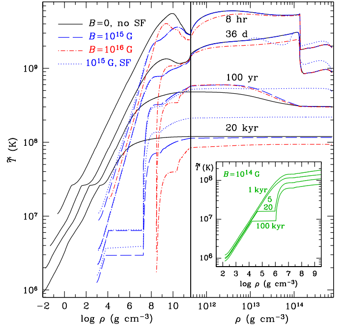
Fig. 11. Redshifted temperature as a function of mass density inside neutrons stars with B = 0 (solid lines), 10^{15} G (long-dashed and dotted lines), and 10^{16} G (dot-dashed lines) at four ages t from 8 h to 2 \times 10^4 yr, marked near the curves. The dotted line illustrates the model with superfluidity SF081322; the other lines are calculated without superfluidity. The two parts of the figure, separated by the vertical solid line, show the regions before and after neutron drip at different density scales. Inset: temperature profiles in the envelopes of a neutron star with B = 10^{14} G at ages t = 1, 5, 20, and 100 kyr.
