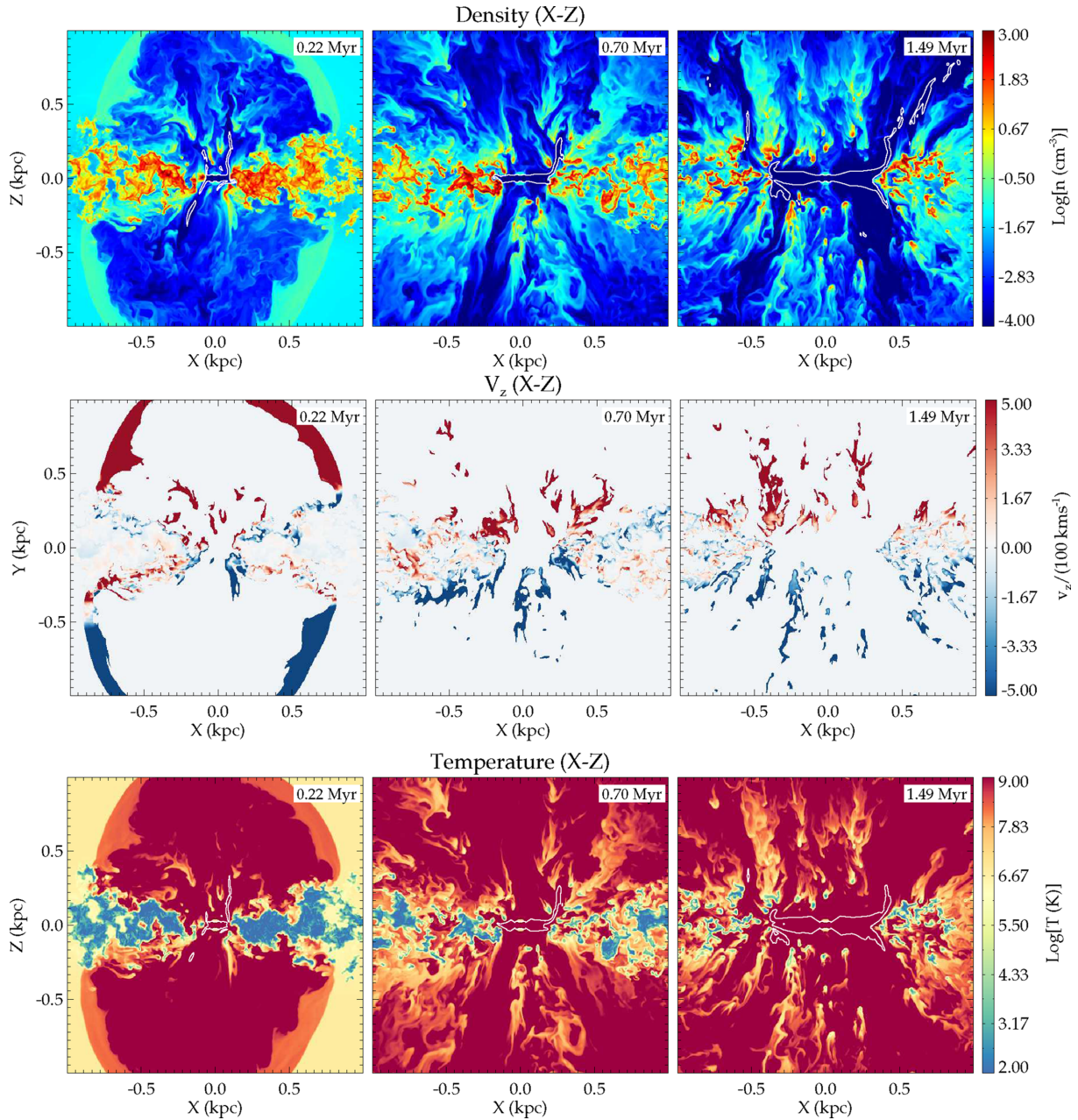
Figure 2. Mid-plane slices in the X - Z plane ( Y = 0 ) of the evolution of simulation P44, for which the jet power is P_{\text{jet}} = 10^{44} erg s ^{-1} . The last column of panels with t = 1.49 Myr corresponds roughly to the current extent of the jets in IC 5063. The top row of panels shows the density ( \log(n[\text{cm}^{-3}]) ), the middle row the vertical component of the velocity ( v_z ) normalized to 100 \text{ km s}^{-1} , for gas with density n > 0.1 \text{ cm}^{-3} , and the bottom row shows the temperature. The white line corresponds to the contours of jet tracer with value 0.1 (maximum being 1), demarcating the region with non-thermal plasma.
