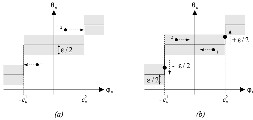
Figure 8 – Pseudo-flow.
