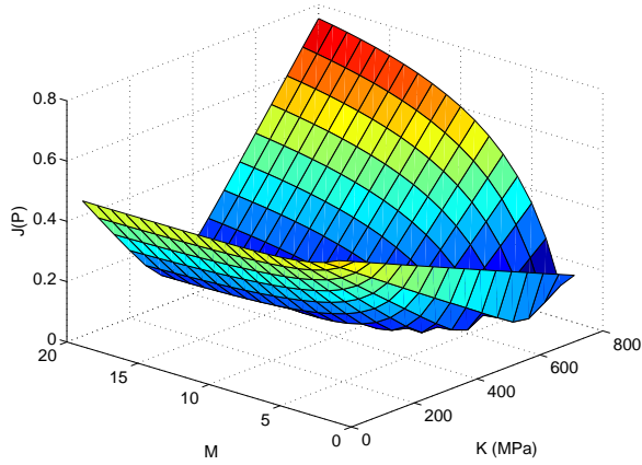
FIGURE 6. Evolution of the cost function versus the material parameters (Ramberg-Osgood law)
