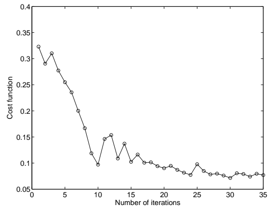
FIGURE 9. Evolution of the cost function over the number of iterations for a weight parameter of 0.9 and the Ramberg-Osgood law
