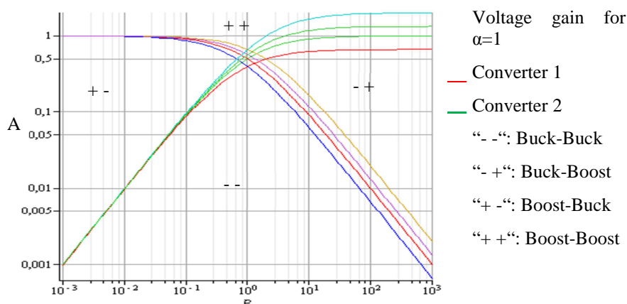
Fig. 7. 2D section of the Fig. 4 for \alpha=1 and V_{in1} \neq V_{in2}
