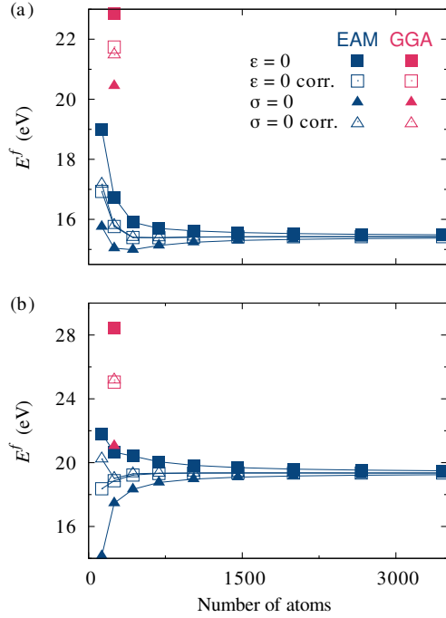
Figure 6: Formation energy of a SIA cluster containing eight interstitials in bcc iron calculated for fixed periodicity vectors ( \bar{\varepsilon} = 0 ) or at zero stress ( \sigma = 0 ) for different sizes of the simulation cell: (a) C15 aggregate and (b) parallel-dumbell configuration with a \langle 111 \rangle orientation. Atomistic simulations are performed either with the M07 empirical potential [101] (EAM) or with ab initio calculations (GGA). Filled symbols refer to uncorrected results and open symbols to the results corrected by the elastic model (see Ref. [99] for more details).
