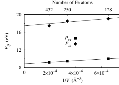
Figure 3: Elastic dipole of a C atom lying in a [001] octahedral interstitial site in bcc Fe as a function of the inverse volume V of the supercell. The elastic dipole has been deduced from the residual stress in ab initio calculations (see Ref. [47] for more details).
