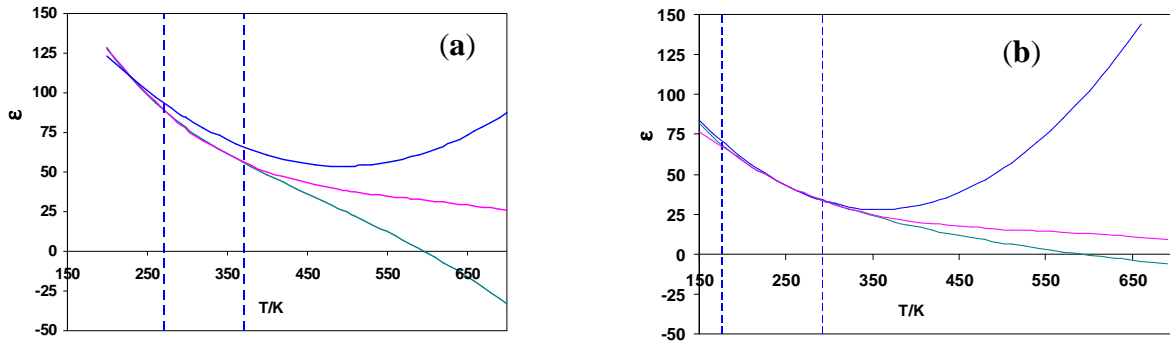
Fig. 2. Relative permittivity \epsilon_r , with respect to temperature: (a) H 2 O and (b) methanol. Calculations: (—) this work, (---) literature (a) [26], (b) [27], (---) CRC tables [28]. Limit of the experimental domain (---) [28].
