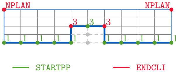
Fig. 4: Sketch of the starting and ending plane number for lateral boundary nodes of vertical structures (STARTPP and ENDCLI respectively). The grey circles represent the ignored nodes whereas the dashed line the ignored elements.
