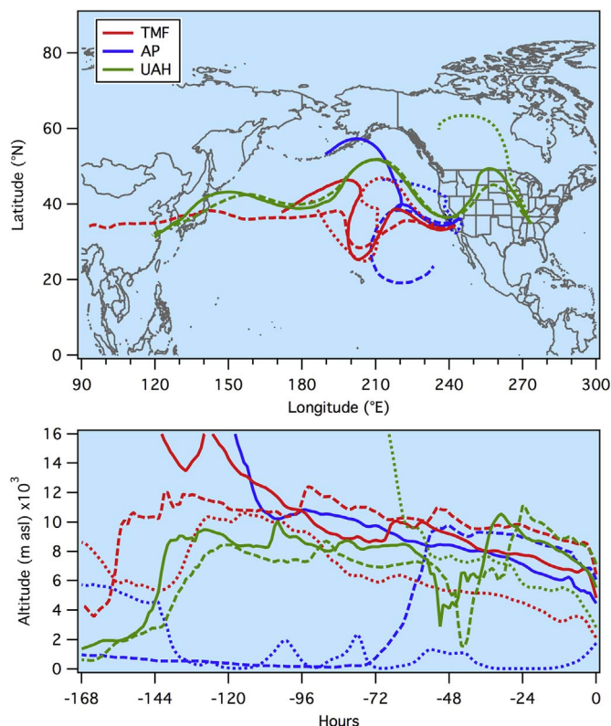
Fig. 7. Complete 7-day HYSPLIT back trajectories (0.5° GDAS meteorology) launched from TMF (red), AP (blue), and UAH (green). The dotted, solid, and dashed lines correspond to launch pressure altitudes of 700, 500, and 400 hPa. (For interpretation of the references to colour in this figure legend, the reader is referred to the web version of this article.)
