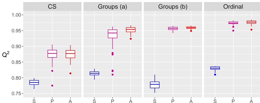
Figure 8: Q^2 of several GP models, based on 60 random designs, corresponding to different model choices for the chemical element. First panel: Single group. Second panel: 5 groups, with a common between-group covariance. Third panel: 5 groups. Fourth panel: Ordered levels. For each panel, three combinations of kernel are tested: sum (S), product (P) or ANOVA (A). Total number of parameters used (panel order): ‘prod’ = (12, 21, 30, 14), ‘sum’ = ‘prod’ + 6, ‘anova’ = ‘prod’ + 7.
