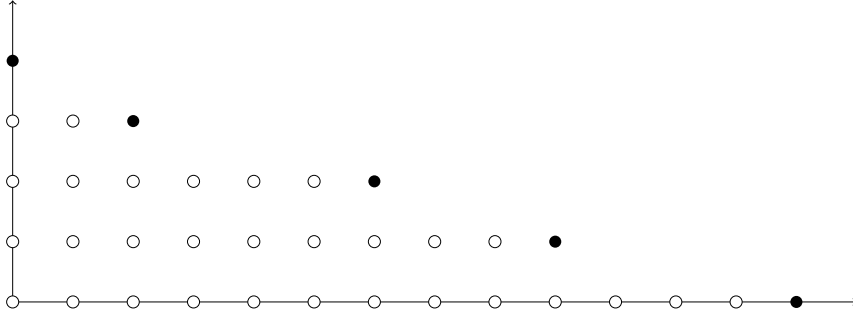
Figure 1. An vanilla Gröbner stairs with respect to \prec_4 ( D=30, n=4, q=1, r=2 ).
