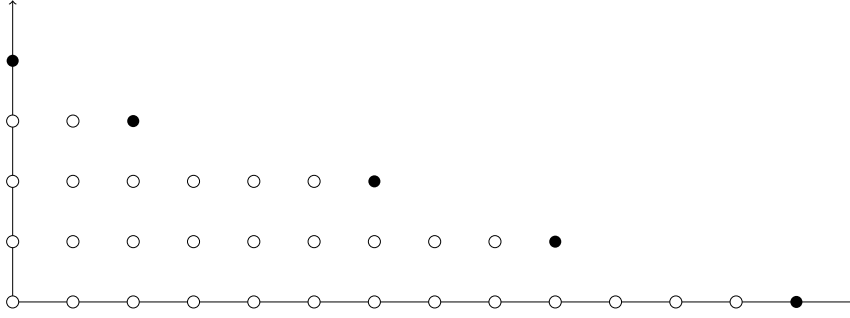
Figure 1. An vanilla Gröbner stairs with respect to <_4 ( D=30, n=4, q=1, r=2 ).
