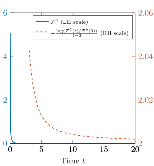
(C) Evolution of the Linearized Entropy \mathcal{F}^\delta , ie the square of the \ell^2(\mu^{\delta v} \delta v) -norm of f (left) and of the Fisher information \mathcal{G}^\delta defined in (11) (right). In each plot, the left-hand scale (plain line) is the linear scale and the right-hand scale (dashed line) is the "-log/t" scale that shows the numerical rate of convergence in long time.
