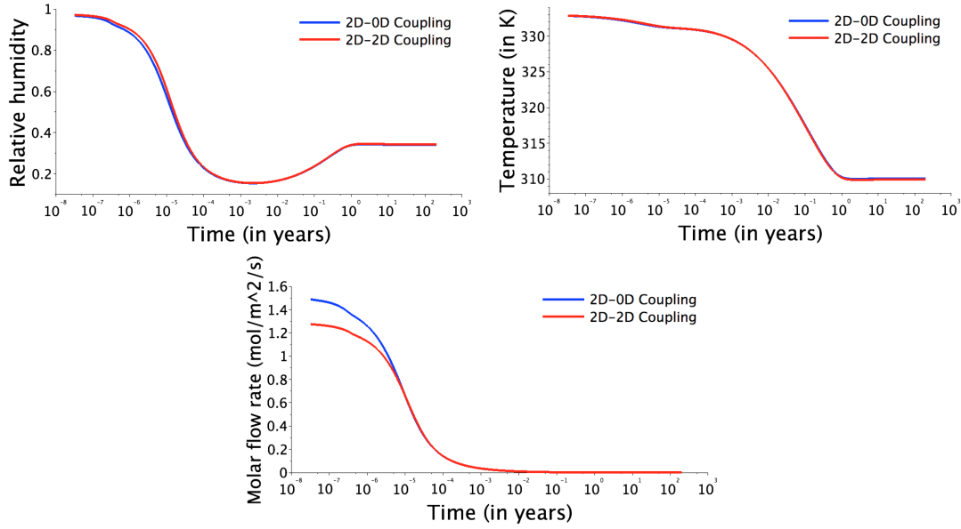
Fig. 5.5 Mean relative humidity, mean temperature (in K) and molar flow rate of the water component (in \text{mol}\cdot\text{m}^{-2}\cdot\text{s}^{-1} ) at the interface as a function of time (in years) for both models with T_{pm}^0 = 333 K and N_y = 90 .
