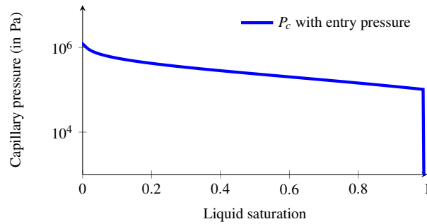
Fig. 6.6 Capillary pressure (in Pa) with a non-zero entry pressure as a function of the liquid saturation.
