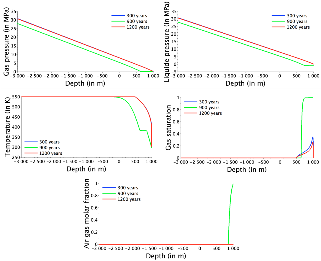
Fig. 6.5 Gas and liquid pressures (in MPa), temperature (in K) and gas saturation as functions of depth (in m) and air molar fraction in the gas phase obtained at times t = 300 years, 900 years and 1200 years for the dependent on time input molar flow rate.
