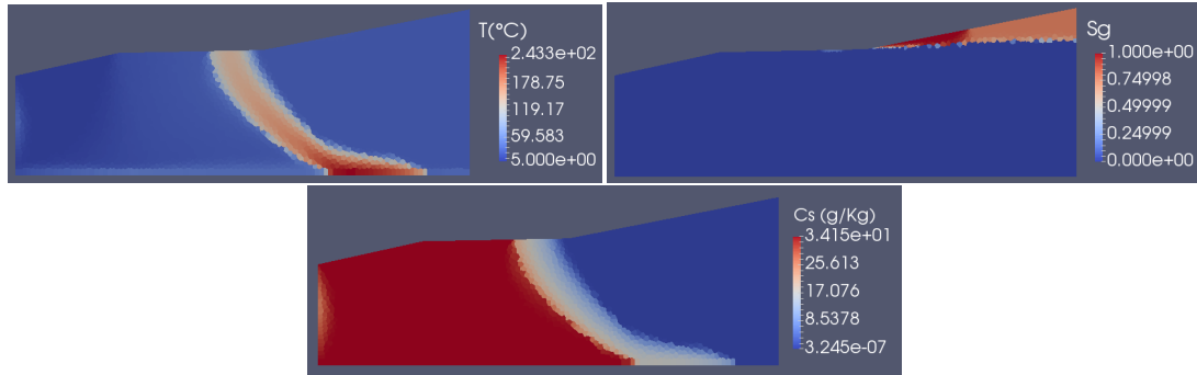
Fig. 6.12 Temperature (in Celsius), gas saturation and salinity of the liquid phase (in g.Kg^{-1} ) at final time (1000 years) obtained with the fine mesh and the air-water-salt test case.
