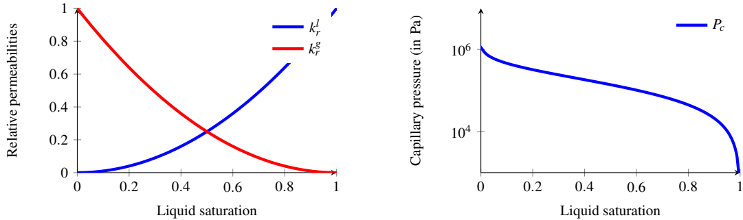
Fig. 6.1 Relative permeabilities (left) of both phases k_r^\alpha , \alpha = g, l and capillary pressure P_c (right) as functions of the liquid saturation S^l .
