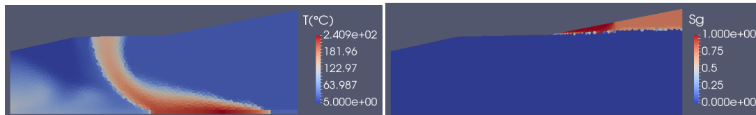
Fig. 6.11 Temperature (in Celsius) and gas saturation at final time (1000 years) obtained with the fine mesh and the evaporation-outflow boundary condition.
