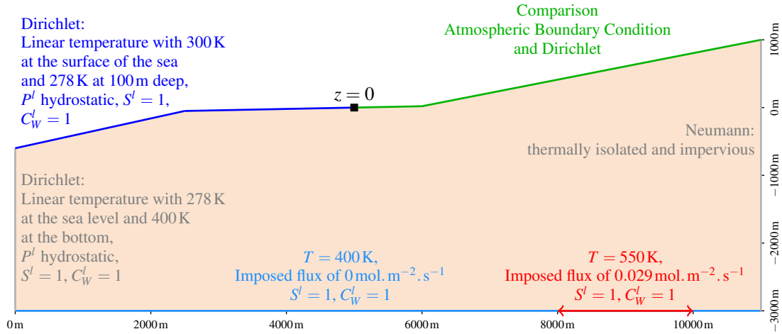
Fig. 6.9 Illustration of the two dimensional domain and its boundary conditions.
