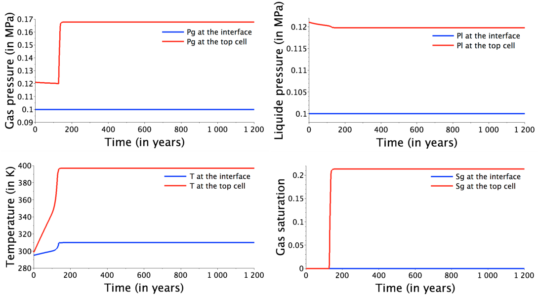
Fig. 6.8 Gas and liquid pressures (in MPa), temperature (in K) and gas saturation at the top boundary and at the top cell as functions of time.
