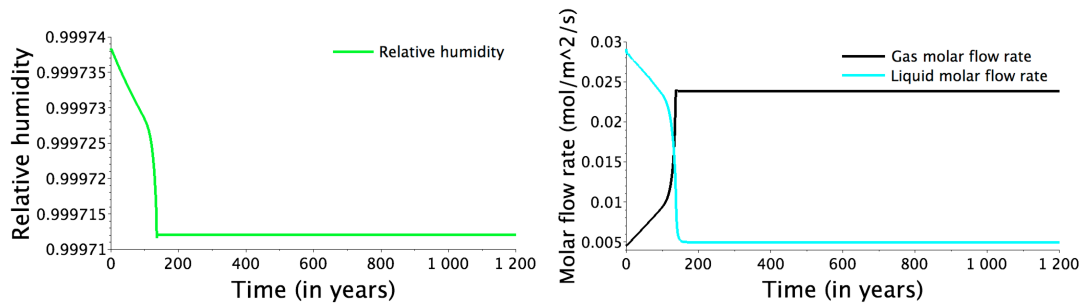
Fig. 6.7 Relative humidity and gas and liquid molar flow rates (in \text{mol} \cdot \text{m}^{-2} \cdot \text{s}^{-1} ) at the top boundary as functions of time.
