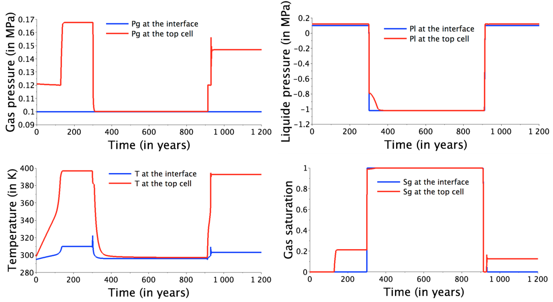
Fig. 6.4 Gas and liquid pressures (in MPa), temperature (in K) and gas saturation as functions of time both at the top boundary and at the top cell, obtained for the dependent on time input molar flow rate.
