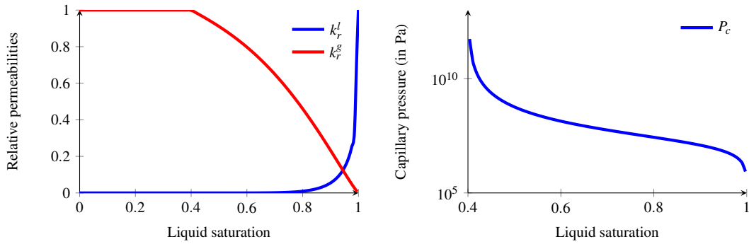
Fig. 5.3 Relative permeabilities (left) of both phases k_r^\alpha , \alpha = g, l and capillary pressure P_c (right) as functions of the liquid saturation S^l of the Callovo Oxfordian clay.
