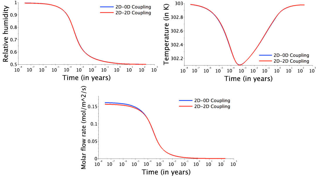
Fig. 5.4 Mean relative humidity, mean temperature (in K) and molar flow rate of the water component (in \text{mol} \cdot \text{m}^{-2} \cdot \text{s}^{-1} ) at the interface as a function of time (in years) for both models with T_{pm}^0 = 303 \text{ K} and N_y = 90 .
