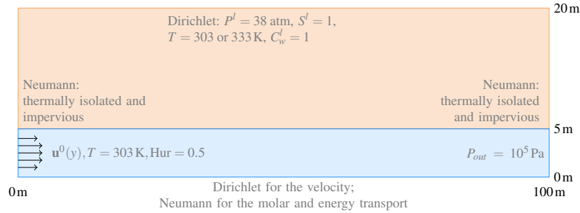
Fig. 5.1 Computational domain of the coupled Darcy and full-dimensional free-flow models.
