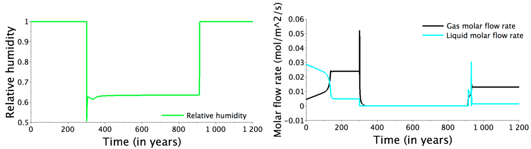
Fig. 6.3 Relative humidity and gas and liquid molar flow rates (in \text{mol} \cdot \text{m}^{-2} \cdot \text{s}^{-1} ) as functions of time, obtained for the dependent on time input molar flow rate.
