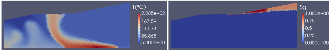
Fig. 6.10 Temperature (in Celsius) and gas saturation at final time (1000 years) obtained with the fine mesh and the Dirichlet top boundary conditions.
