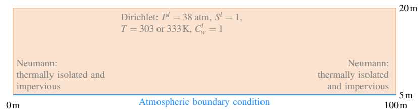
Fig. 5.2 Computational domain of the Darcy flow model coupled with the soil-atmosphere evaporation-outflow boundary condition.
