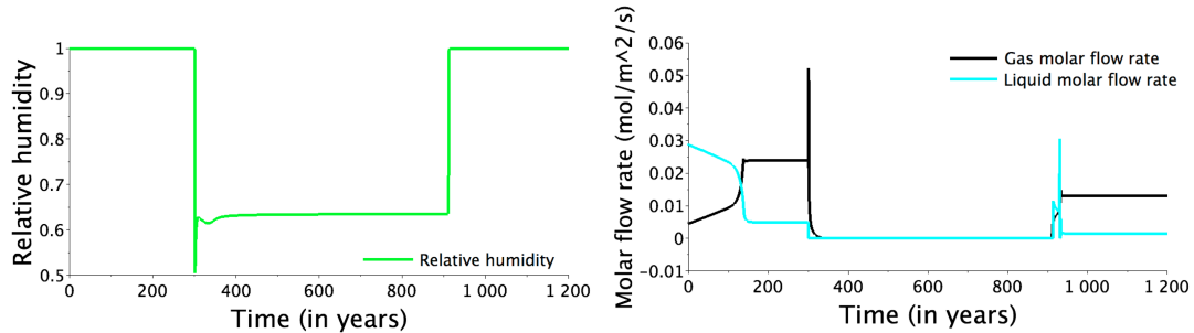
Fig. 6.3 Relative humidity and gas and liquid molar flow rates (in \text{mol} \cdot \text{m}^{-2} \cdot \text{s}^{-1} ) as functions of time, obtained for the dependent on time input molar flow rate.
