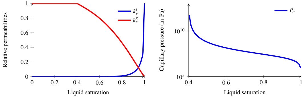
Fig. 5.3 Relative permeabilities (left) of both phases k_r^\alpha , \alpha = g, l and capillary pressure P_c (right) as functions of the liquid saturation S^l of the Callovo Oxfordian clay.
