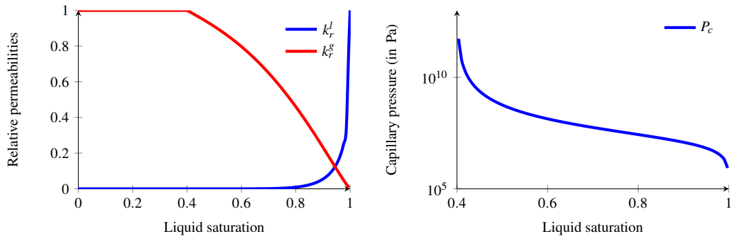
Fig. 6.3 Relative permeabilities of both phases k_r^\alpha , \alpha = g, l and capillary pressure P_c as functions of the liquid saturation S^l of the Callovo Oxfordian clay.
