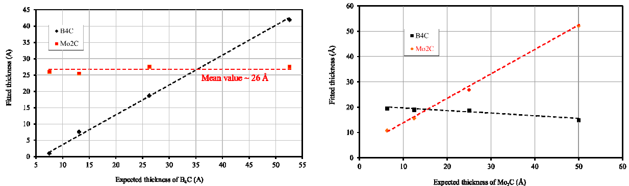
Figure3. Variation of B_4C and Mo_2C fitted thicknesses as function of B_4C expected thickness (left), for a Mo_2C thickness fixed at 2.5 nm. Variation of B_4C and Mo_2C fitted thicknesses versus Mo_2C expected thickness (right), for a B_4C thickness fixed at 2.5 nm.
