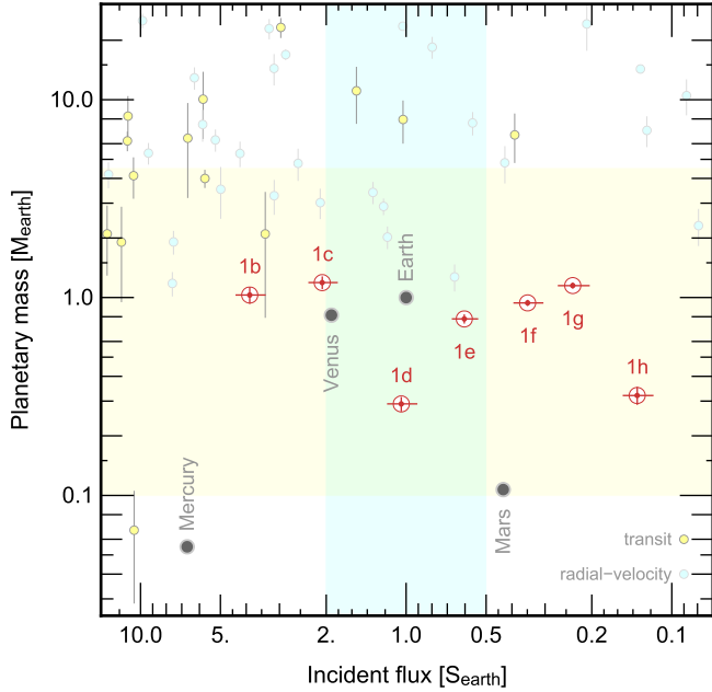
Fig. 12. Masses and the incident fluxes received by the TRAPPIST-1 planets, compared to other exoplanets found by the transit method (yellow), via the radial-velocity technique (blue), and to the terrestrial worlds of the Solar system (grey). We highlight two ranges of interest in mass and incident flux. All objects contained in the exoplanet.eu catalogue (Schneider et al. 2011), found by the RV, or the transit method, are included in this figure.
