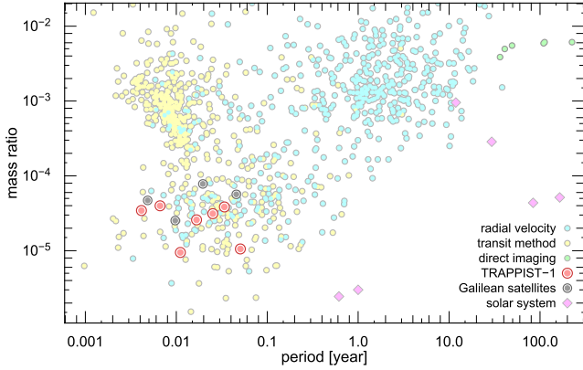
Fig. 11. Ratio between the mass of a planet or moon and that of its host as a function of orbital period. We represent the known population of exoplanets (from exoplanet.eu, Schneider et al. 2011) from three different detection methods. The Solar system is also highlighted. The TRAPPIST-1 system, like the Galilean moons of Jupiter, share a similar parameter space with the sub-Neptune and super-Earth population. Orbital periods are used to reveal the various sub-populations.
