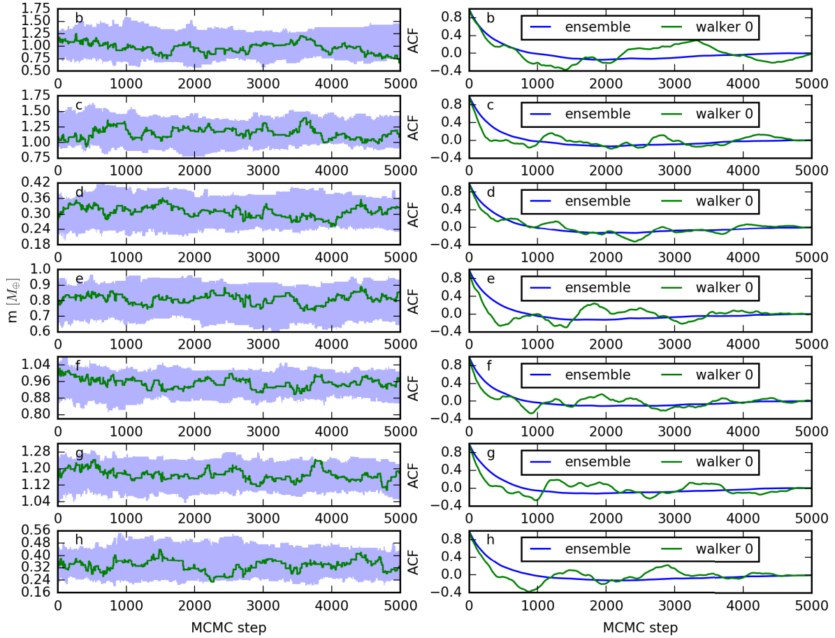
Fig. 5. Left panels: evolution of the masses of all planets of the entire ensemble of 100 walker chains in blue, and the evolution of a single chain in green. Right panels: auto-correlation function of the masses for the ensemble and a single chain.
