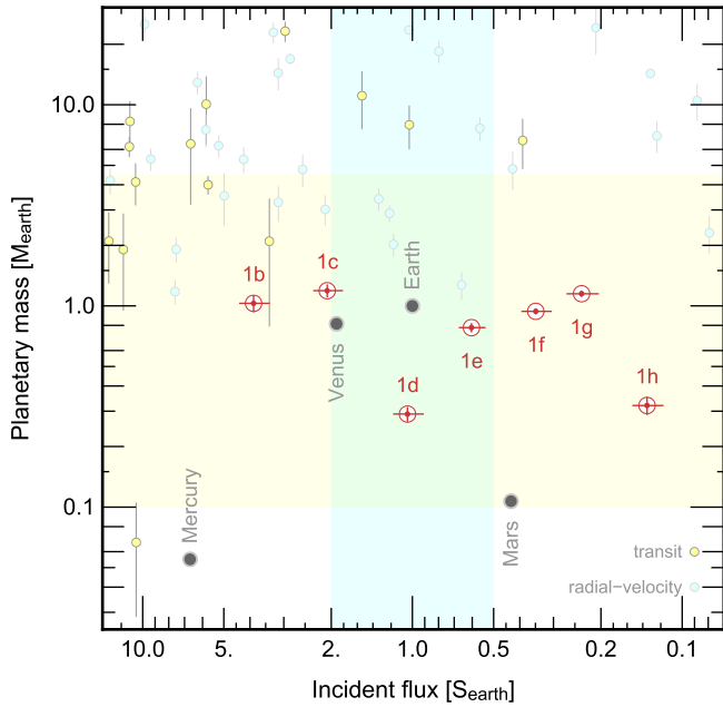
Fig. 12. Masses and the incident fluxes received by the TRAPPIST-1 planets, compared to other exoplanets found by the transit method (yellow), via the radial-velocity technique (blue), and to the terrestrial worlds of the Solar system (grey). We highlight two ranges of interest in mass and incident flux. All objects contained in the exoplanet.eu catalogue (Schneider et al. 2011), found by the RV, or the transit method, are included in this figure.
