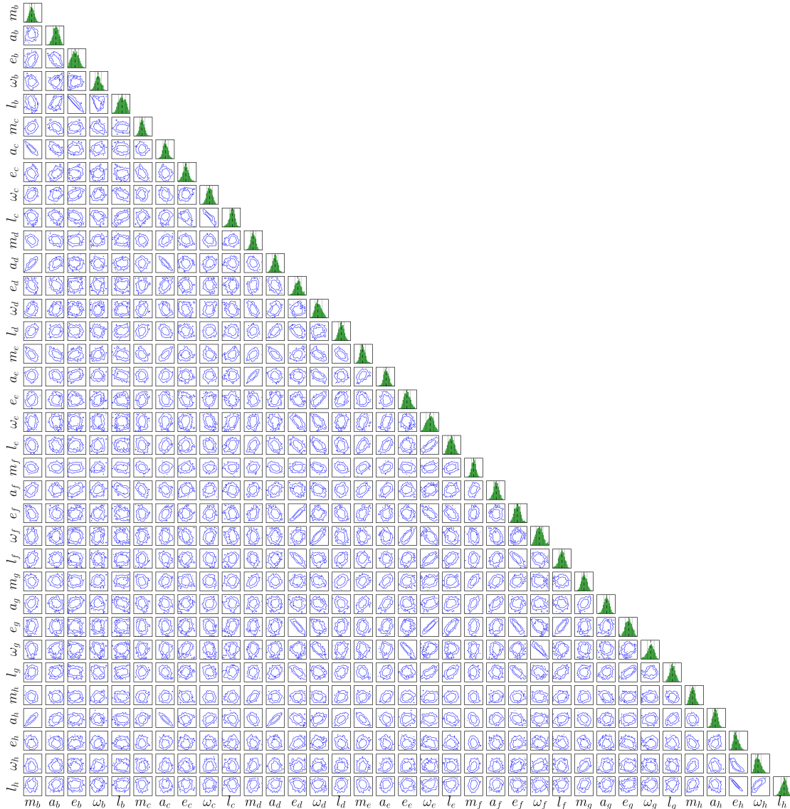
Fig. 6. Posterior probability distribution between all pairs of parameters, the masses m , the semi-major axes a , the eccentricities e , the arguments of perihelion \omega , and the mean longitudes l = \Omega + \omega + M of all seven planets. It is showing strong correlations between many pairs of parameters, especially between m and a and between e and \omega .
