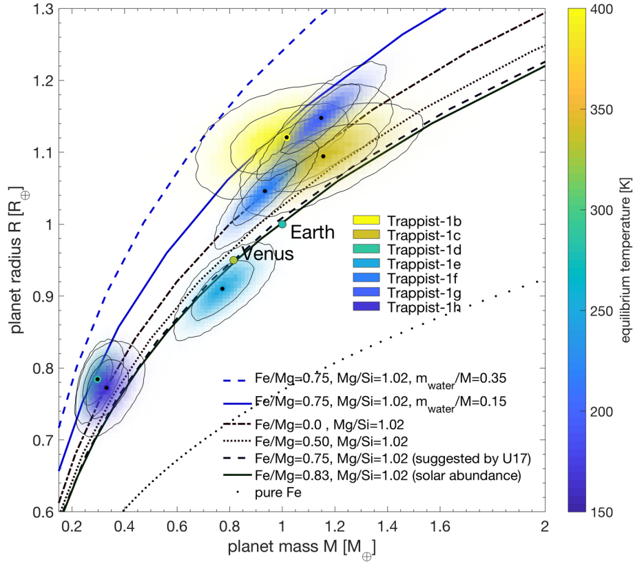
Fig. 10. Mass–radius diagram for the TRAPPIST-1 planets, Earth, and Venus. Curves trace idealised compositions of rocky and water-rich interiors (surface temperature fixed to 200 K). Median values are highlighted by a black dot. Coloured contours correspond to significance levels of 68% and 95% for each planet. The interiors are calculated with model II of Dorn et al. (2017). Rocky interiors are composed of Fe, Si, Mg, and O, assuming different bulk ratios of Fe/Mg and Mg/Si. U17 refers to Unterborn et al. (2018). Equilibrium temperatures for each planet are indicated by the coloured contours.
