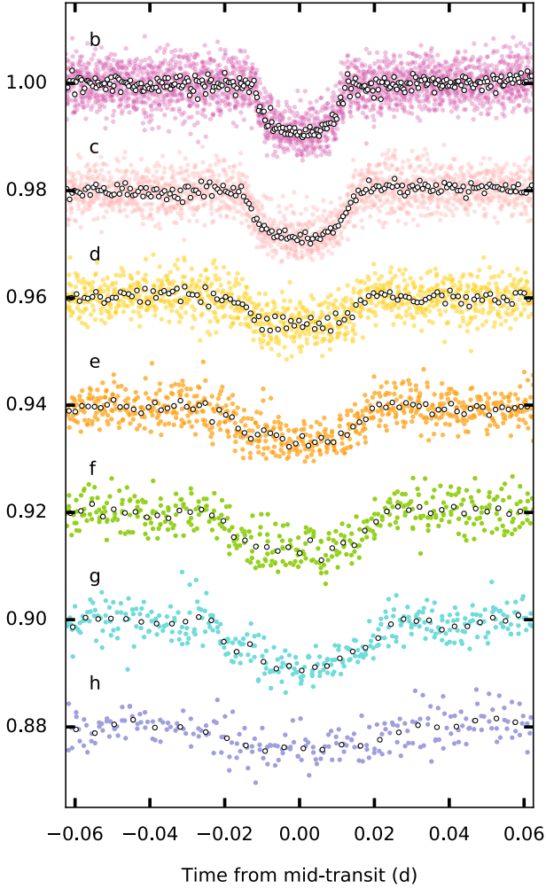
Fig. 1. Folded short-cadence lightcurves extracted from K2 data, corrected for their corrected for their TTVs. Relative fluxes are shown for each planet and are shifted vertically for clarity. The short-cadence data are binned to produce the coloured points, with five cadences per point. The white points are further binned, with ten points taken from the folded curve per bin.
