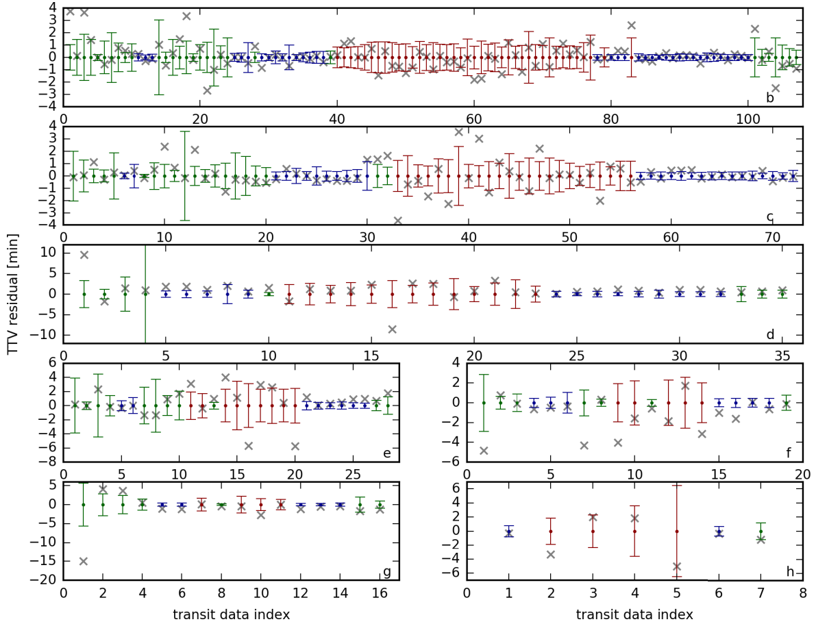
Fig. 3. Residuals of the TTVs shown in Fig. 2. The transit data index corresponds to the column index of Tables A.1–G.1.
