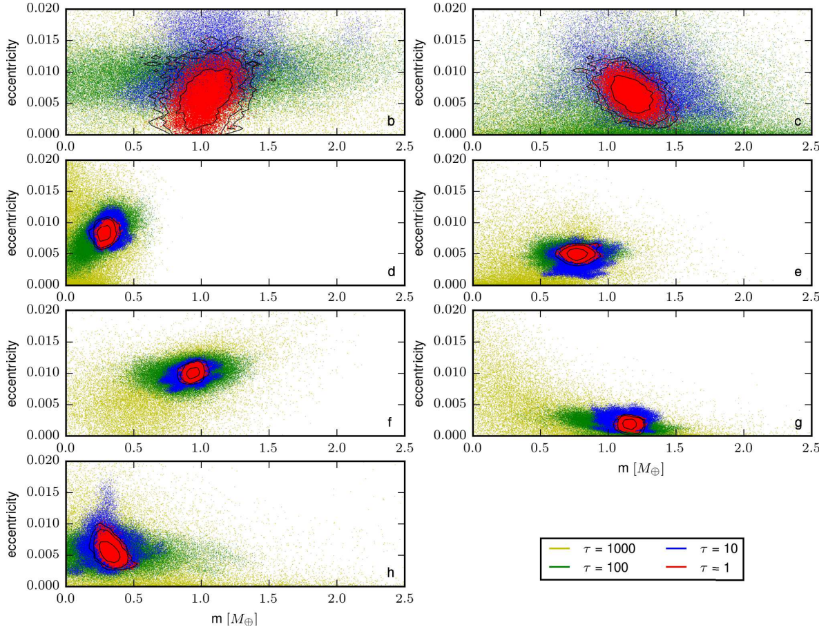
Fig. 4. Posterior probability distribution of the mass and eccentricities of all seven planets, for different MCMC sampling “temperatures” \tau , assuming a stellar mass of M_{\star} = 0.09 M_{\odot} (Van Grootel et al. 2018). The contours correspond to significance levels of 68%, 95% and 99% for \tau = 1 . Sampling “temperatures” greater than one are used to cover a larger parameter space.
