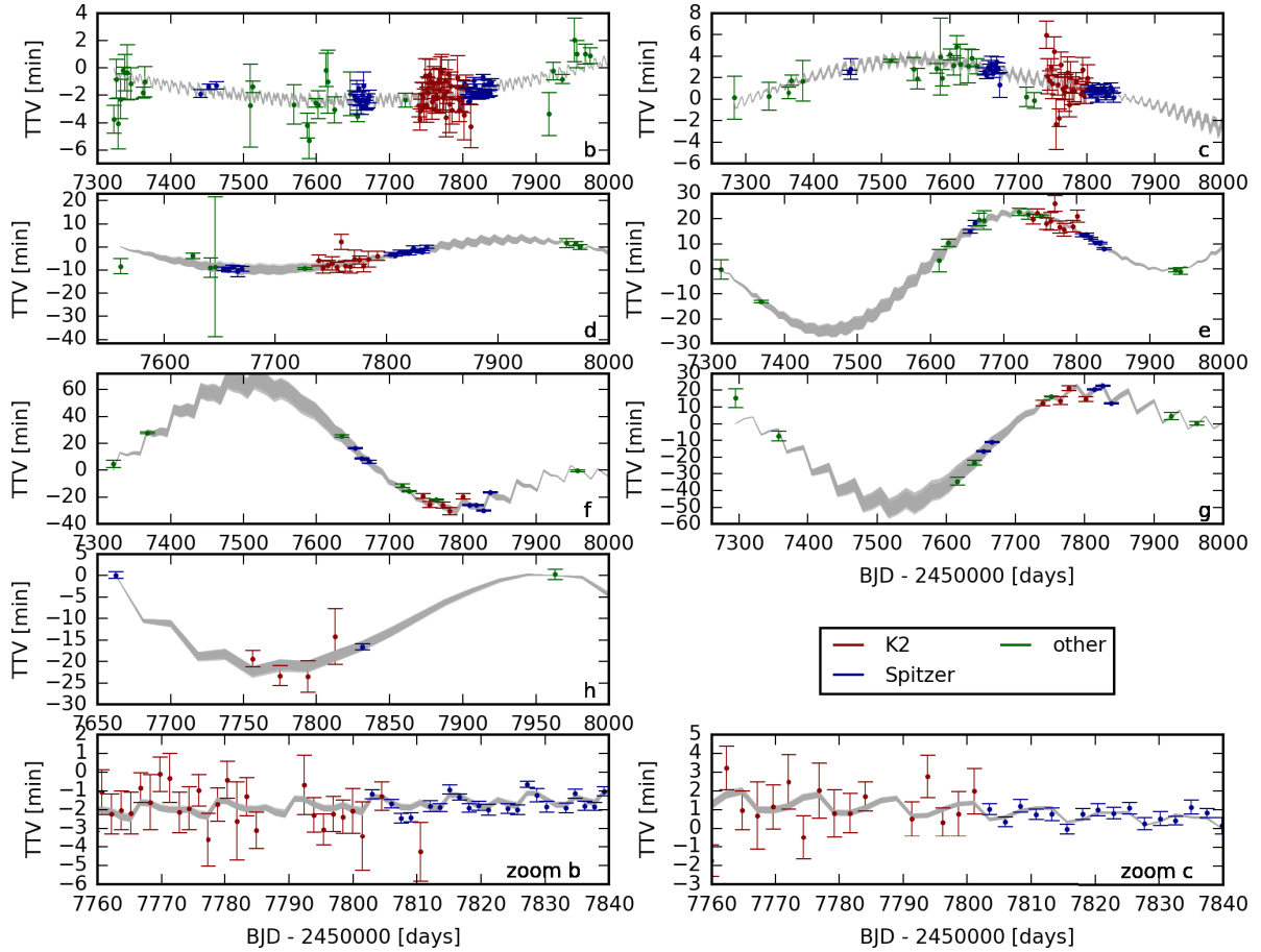
Fig. 2. Calculated TTVs for all planets and for 1000 different MCMC samples (grey lines). Measured transit times with the corresponding uncertainties are indicated by coloured symbols, according to the used telescope. A detailed list of all transits is given in Appendix. The differences between the solutions reflect the distribution shown in Fig. 4 for \tau = 1 . The two panels at the bottom show a zoomed region for planet b and c.
