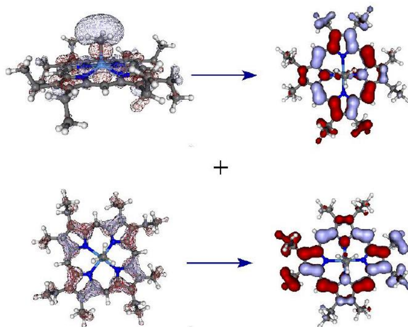
Figure 8: Natural transition orbitals of the Q band (doubly-degenerated) excitation
