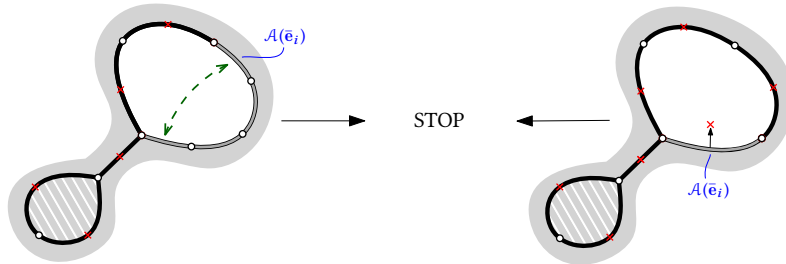
Figure 6: The two ways Algorithm 1 may stop. (Left) The \theta -th peeling step identifies A(\bar{e}_{\theta-1}) with the edge adjacent immediately on the right of the black segment. Then, we fill-in the “free” hole created. (Right) At time \theta - 1 the boundary of \bar{e}_{\theta-1} contains a single free edge which is then given a mark at step \theta and becomes black. In both cases, the boundary of \bar{e}_\theta is completely black, and the algorithm stops.
