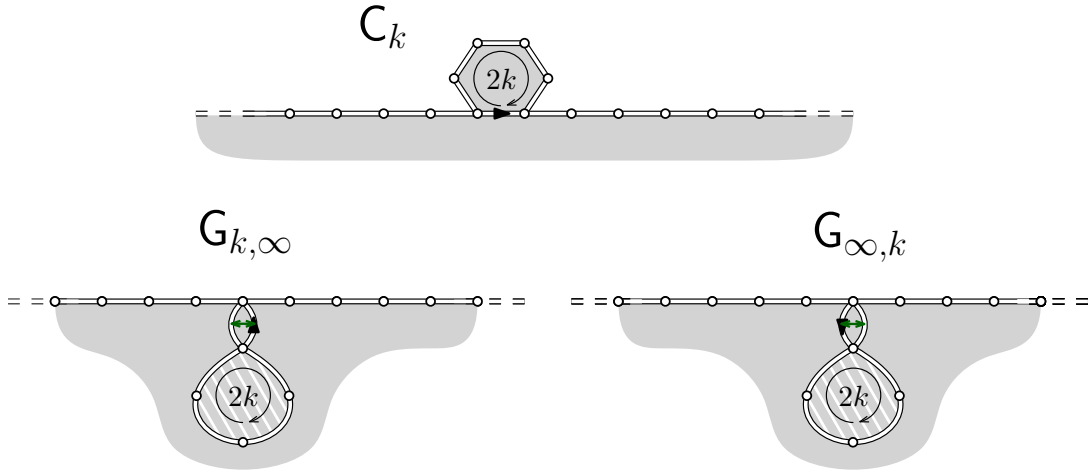
Figure 8: The peeling events C_k , G_{k,\infty} and G_{\infty,k} . On the event C_k , the face f_i does not belong to \bar{e}_i , and has degree 2k ( k \in \mathbb{N} ). In this case, \bar{e}_{i+1} is obtained from \bar{e}_i by adding this new face, without performing any identification of its edges. Otherwise, f_i belongs to \bar{e}_i and \bar{e}_{i+1} is obtained from \bar{e}_i by identifying the two half-edges of the hole that correspond to \mathcal{A}(\bar{e}_i) . This creates two holes, one of which is infinite. We denote this event by G_{k,\infty} (if we identify \mathcal{A}(\bar{e}_i) to an edge on its left) or G_{\infty,k} (in the other case), where 2k ( k \in \mathbb{Z}_{\geq 0} ) stands for the perimeter of the finite hole.
