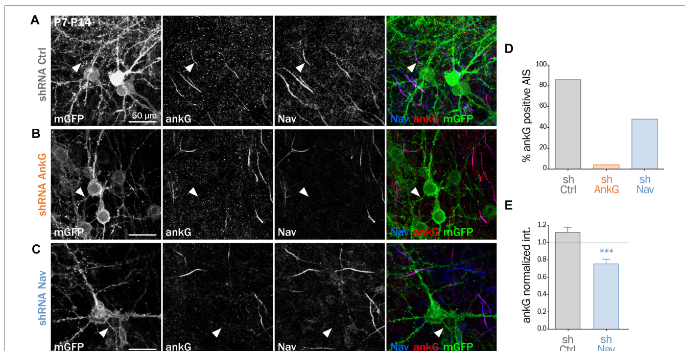
FIGURE 1 | Knockdown of Nav channels downregulates the axon initial segment (AIS) in organotypic slices. Organotypic cortical slices prepared from postnatal day 7 rats were infected with a lentivirus co-expressing membranous GFP (mGFP) and shRNA directed against ankG (shAnkG), Nav (shNav) or luciferase as control (shCtrl). Seven days post-infection, slices were fixed, immunostained for GFP, ankG and Nav. (A–C) Maximum intensity projection of 15–20 optical slices. Scale bar: 50 \mu m. (D) Percentage of infected neurons with an observable AIS (shCtrl n = 80 ; shAnkG n = 27 ; shNav n = 97 ; sum of three independent experiments). (E) Ratio of the mean fluorescence intensity for ankG labeling at the AIS in transfected neurons (where the AIS was still detected) compared to the surrounding untransfected cells (shCtrl 1.10 \pm 0.06 , n = 69 ; shNav: 0.72 \pm 0.05 , n = 47 ; three independent experiments).
