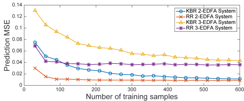
Fig. 4. Reduction of the ML models' prediction MSEs of power STDEV with increasing training data size.
