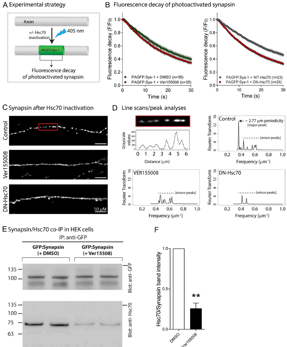
Figure 7. Inactivation of Hsc70 ATPase activity leads to disruption of axonal synapsin. (A) Strategy to analyze the fluorescence decay of PAGFP: synapsin in an axon ROI over time. PAGFP: synapsin was photoactivated in a discrete axonal ROI, and the dispersion of fluorescence was quantified over time. (B) Fluorescence decay of PAGFP: synapsin in axon ROIs. Note faster decay of fluorescence upon Hsc70 inactivation. (C) Representative images showing endogenous distribution of synapsin in axons upon pharmacologic and genetic Hsc70 inactivation (VER155008 and Hsc70-DN). Note that the punctate distribution is disrupted upon Hsc70 inhibition. (D) Quantification of the periodicity of axonal synapsin particles with or without Hsc70 inactivation. Periodicity of endogenous synapsin particles (i.e., distances between adjacent puncta) was determined from axonal line scans, as shown in the example (top left; red boxed region from C). Cumulative data from control axons is shown on the top right, represented by FFTs (see the Colocalization analysis of widefield images... section of Materials and methods for details). Note the major peak at \sim 2.77 \mu\text{m} , representing the typical spacing of synapsin puncta in control axons (dashed line over minor peaks). Also note loss of the major peak upon Hsc70 inhibition, reflecting disruption of the periodic synapsin distribution in axons. (E) HEK293 cells were transfected with GFP: synapsin, immunoprecipitated with an anti-GFP antibody, and blotted with anti-GFP and anti-Hsc70 antibodies (with or without VER155008). Note that addition of the Hsc70 inhibitor led to a significant reduction in the amount of immunoprecipitated Hsc70. Molecular mass is shown in kilodaltons. (F) Quantification of blots in E. n = 3 separate experiments. Error bars show means \pm SEM. **, P < 0.01 .
