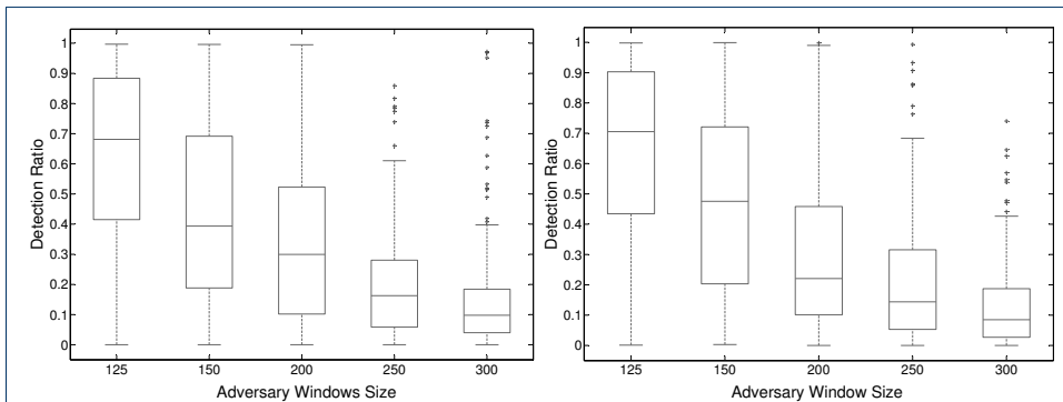
(a) Detection ratio function with respect to the single-watermark against a parametric cyber-physical adversary using different adversary window size for eavesdropping the data of the channel before the attack. (b) Detection ratio function with respect to the multi-watermark against a parametric cyber-physical adversary using different adversary window size for eavesdropping the data of the channel before the attack.
