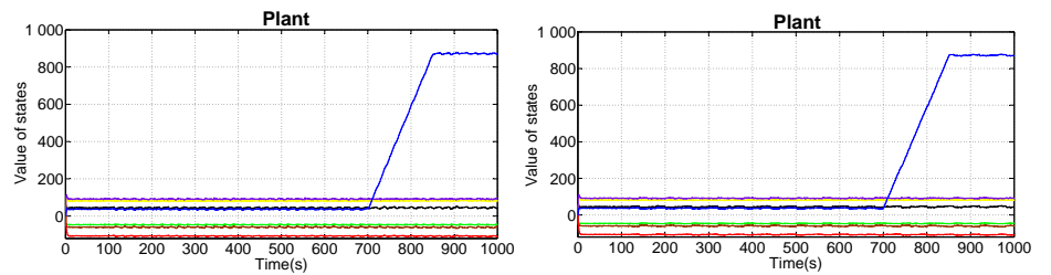
(a) Plant states under a non-parametric cyber-physical adversary attack and switching frequency set to 0.14Hz, adversary attack and switching frequency set to 0.05Hz, i.e., every 7 time steps, the controller changes the distribution associated to the watermark. (b) Plant states under a non-parametric cyber-physical adversary attack and switching frequency set to 0.05Hz, i.e., every 20 time steps, the controller changes the distribution associated to the watermark.
