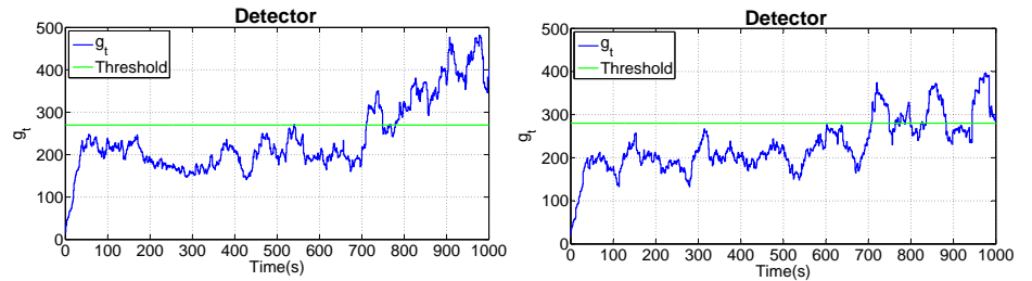
(e) Detector results, switching frequency set to 0.14Hz. (f) Detector results, switching frequency set to 0.05Hz.
