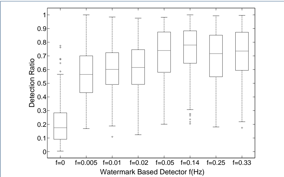
Figure 9 Single ( f = 0 ) and multi ( f = [0.005, 0.01, 0.02, 0.05, 0.14, 0.25, 0.33] ) watermark detector against a non-parametric cyber-physical adversary (the order of the system is 25).
