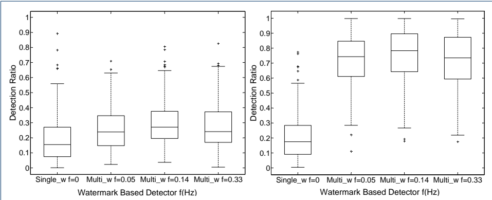
(a) Detection ratio function with respect to the single- and multi-watermark with different switching frequencies for fourth order systems. (b) Detection ratio function with respect to the single- and multi-watermark with different switching frequencies for systems of order 25.
