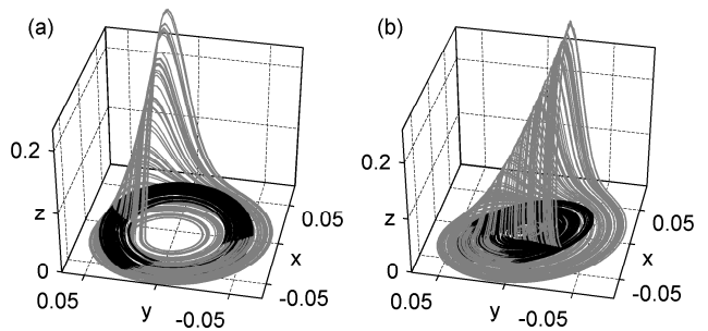
Figure 4. Reconstruction of the leading pair, i. e. RCs 1-2 (black curve), of the coupled Rössler oscillators' actual trajectory (gray curve) in (a) a phase-coherent regime with \alpha = 0.15 ; and (b) in the funnel regime with \alpha = 0.28 .
