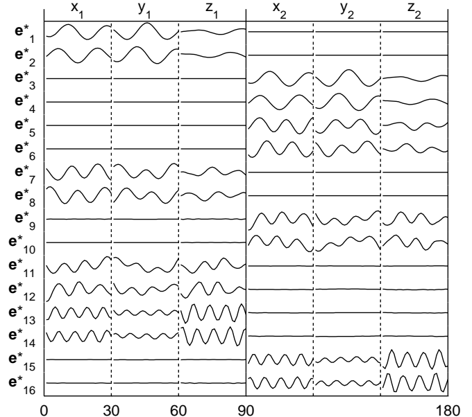
Figure 10. Rotated eigenvectors \mathbf{e}_k^* associated with the 16 largest eigenvalues \lambda_k^* in Fig. 9.
