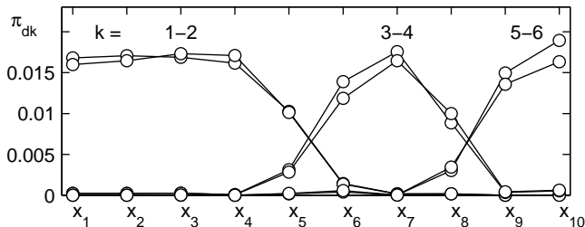
Figure 7. Participation index \pi_{dk} that correspond to Fig. 6. The values for the clusters k = (1,2) , (3,4) and (5,6) are clearly well separated, while intermediate values are assigned to oscillators j = 5 and 8 .
