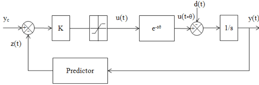
Figure 1. Closed loop scheme of the system including a saturation function
