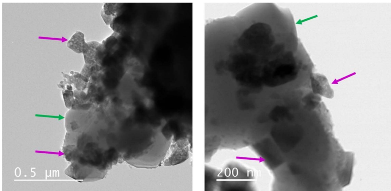
Fig. 4. TEM of Ni/Ca-HA1_S fresh catalyst; → Ni particle, → hydroxyapatite.
