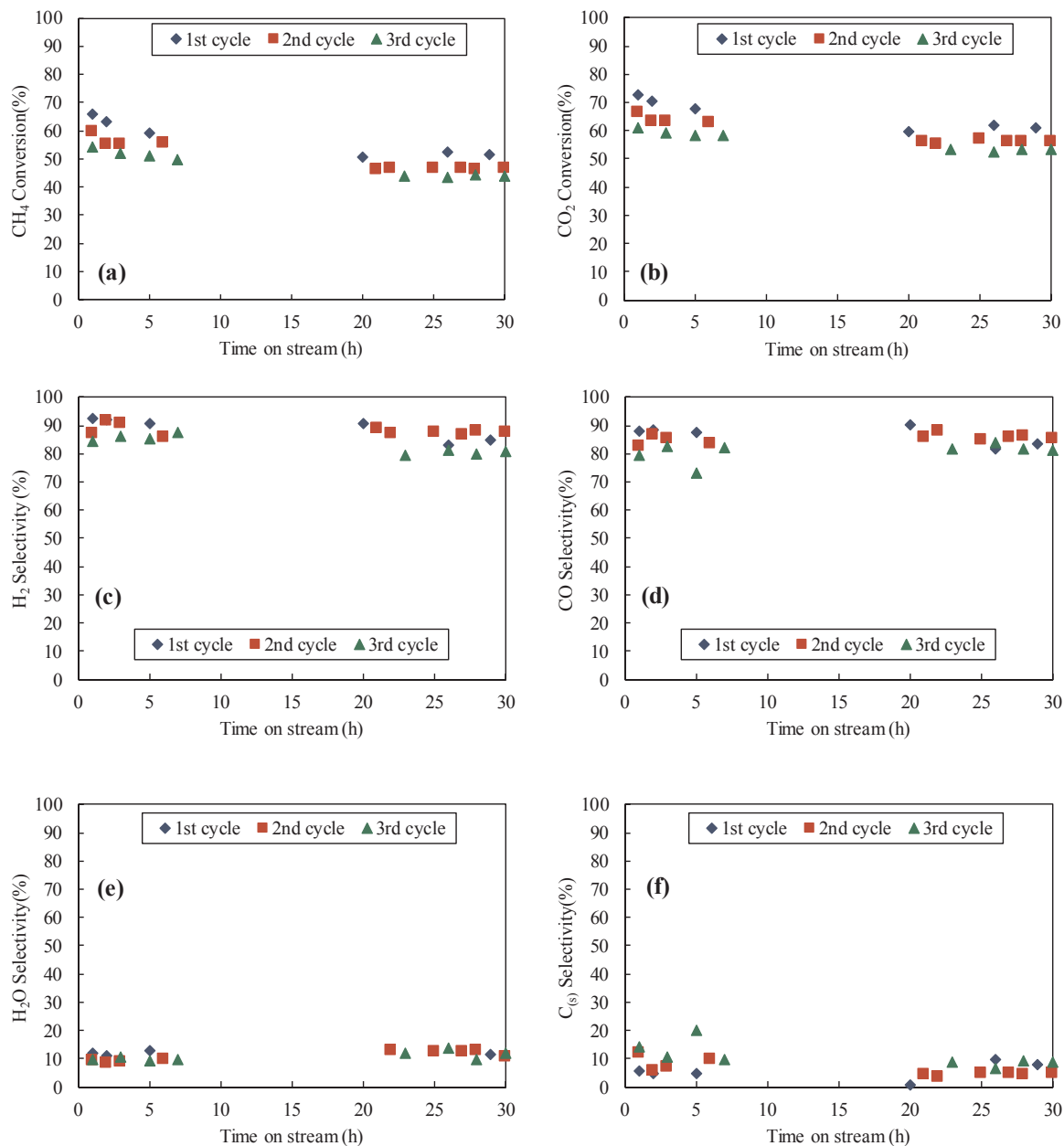
Fig. 6. Catalytic performance of Ni/Ca-HA1_S catalyst under 3 cycles of DRM/Air-regeneration. Reaction conditions: T=700\text{ }^{\circ}\text{C} , \text{WHSV} = 15882\text{ mL h}^{-1}\text{ g}_{\text{cat}}^{-1} , \text{CH}_4/\text{CO}_2 = 1 , \text{TOS}=30\text{ h} . Regeneration conditions: 1\text{h}30 at 700\text{ }^{\circ}\text{C} with air flow.
