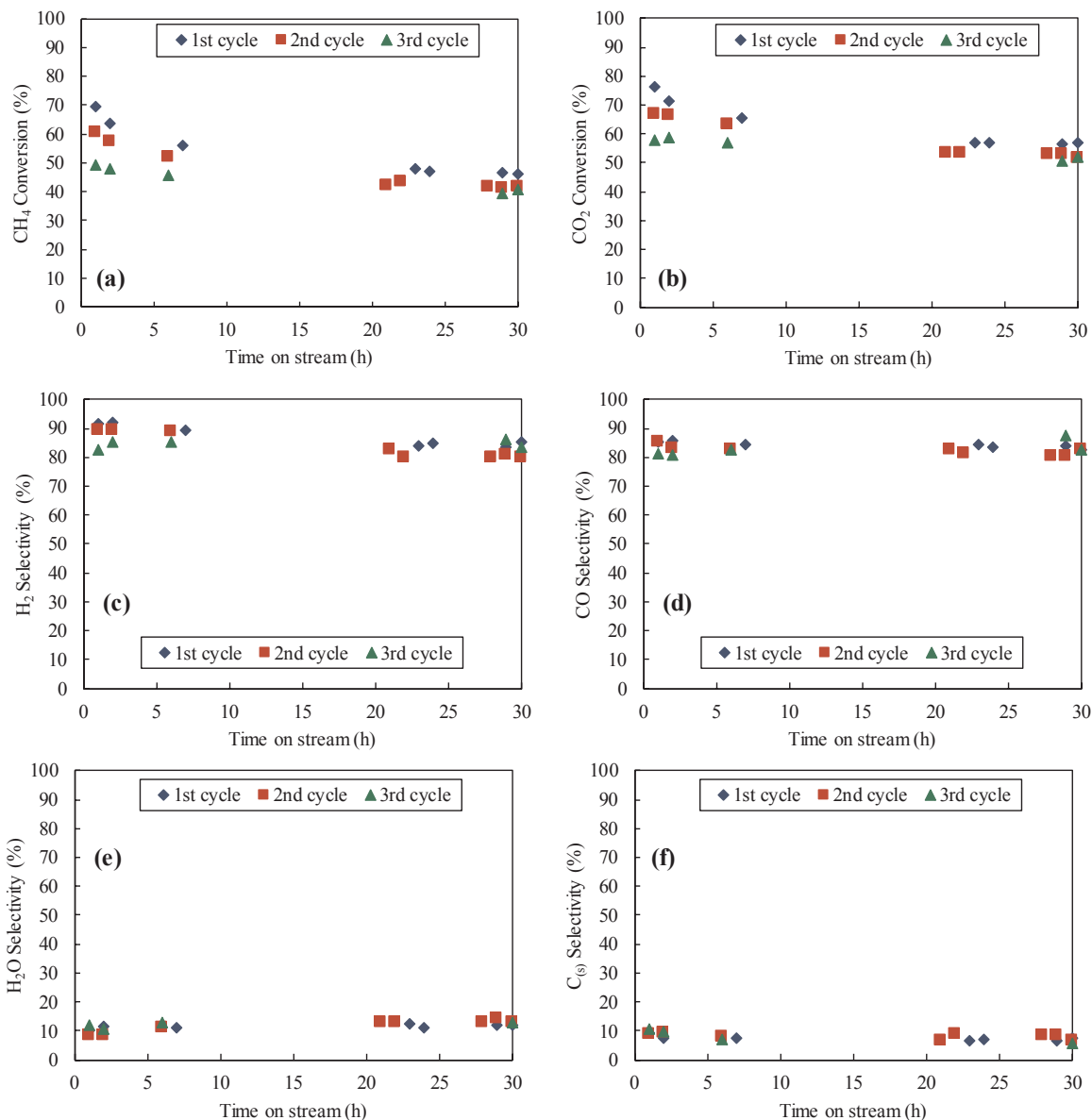
Fig. 8. Catalytic performance of Ni/Ca-HA1_S catalyst under 3 cycles of DRM/CO 2 -regeneration. Reaction conditions: T=700 °C, WHSV = 15882 mL h -1 g cat -1 , CH 4 /CO 2 = 1, TOS=30 h. Regeneration conditions: 1h30 at 700 °C with 21%CO 2 /N 2 flow.
