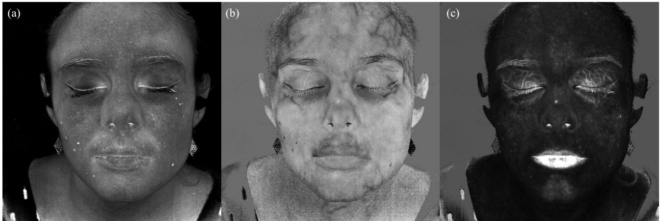
Figure 14. Optical analysis results, volume fraction map of: melanin (a), oxygen (b), blood (c).
