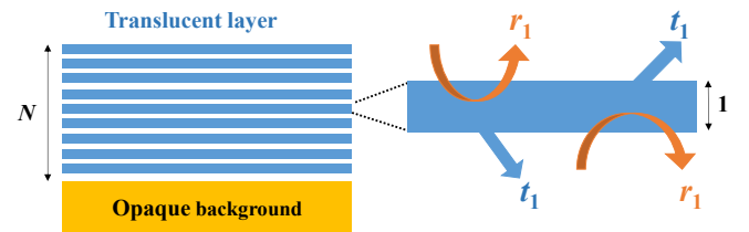
Figure 6. Homogenous translucent layer of thickness N described as the superposition of N identical sub-layers of unit thickness. Two-flux transfers for one unit thickness sub-layer defined by its reflectance r_1 and transmittance t_1 .
