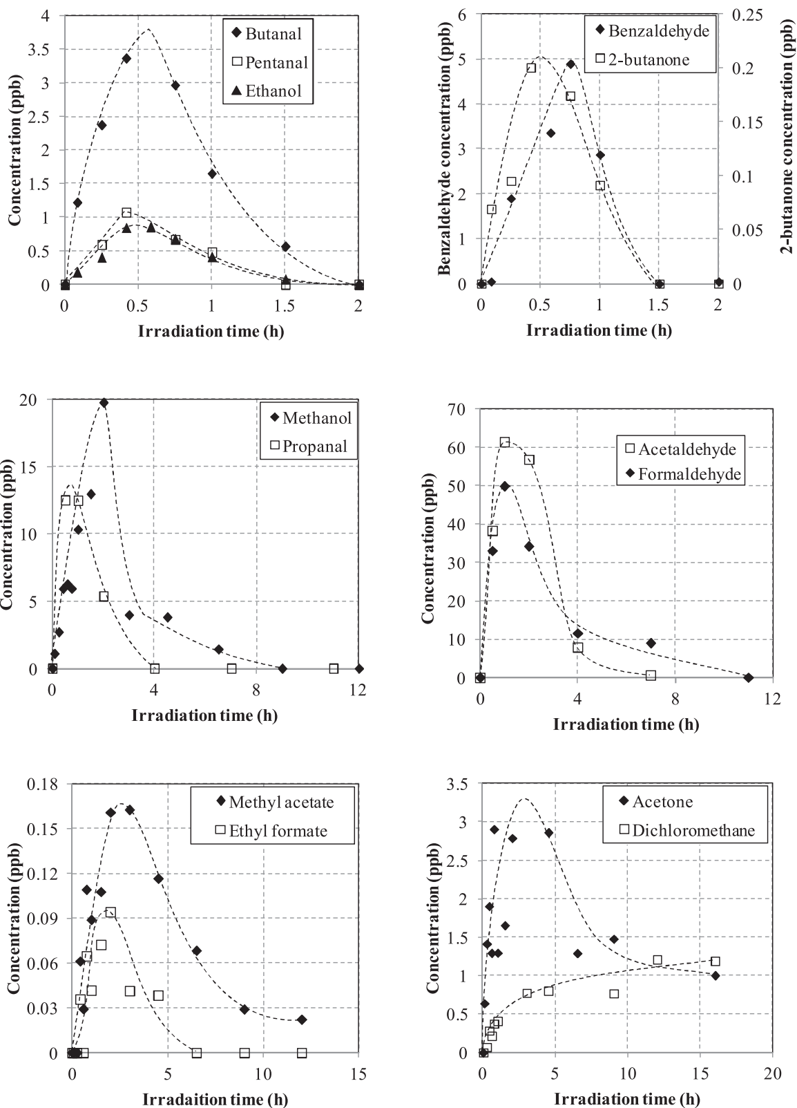
Fig. 11. Time profile curves of intermediates during degradation of toluene, n-decane and TCE in a mixture ( C_{\text{totCO}} = 1228\text{-}1774 ppbv, [\text{H}_2\text{O}] = 13,000 ppm, Q = 28.8 \text{ Nm}^3 \text{ h}^{-1} , I = 0.5 \text{ mW cm}^{-2} ).
