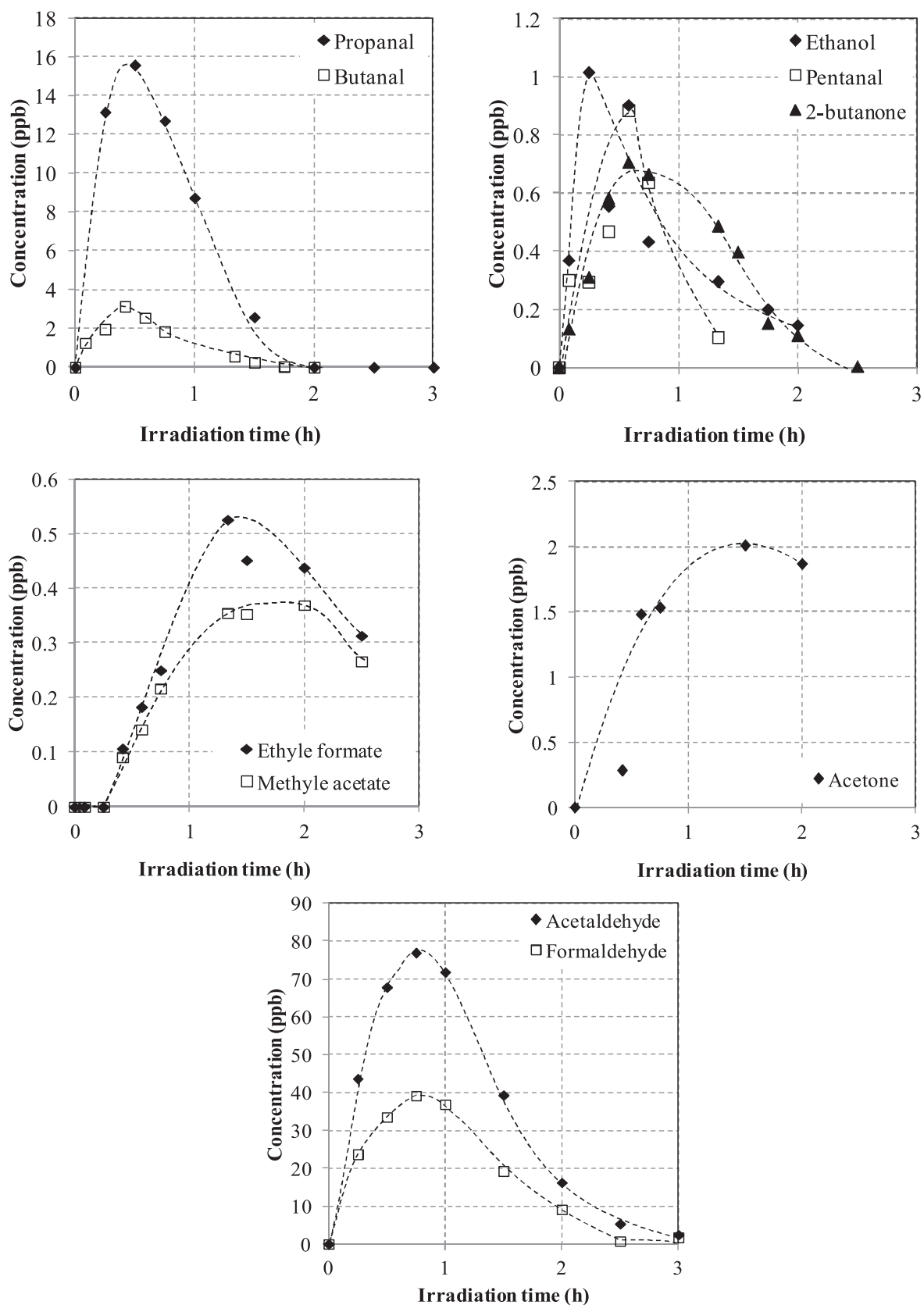
Fig. 6. Time profile concentrations of primary and secondary reaction intermediates during n-decane photocatalytic degradation ( C_{dec0} = 740 ppbv, [H_2O] = 13,000 ppm, Q = 28.8 Nm^3 h^{-1} , I = 0.5 mW cm^{-2} ).
