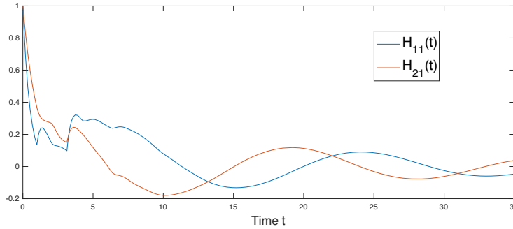
Fig. 1 Graphs of the kernels H_{11}(t) and H_{21}(t) .
