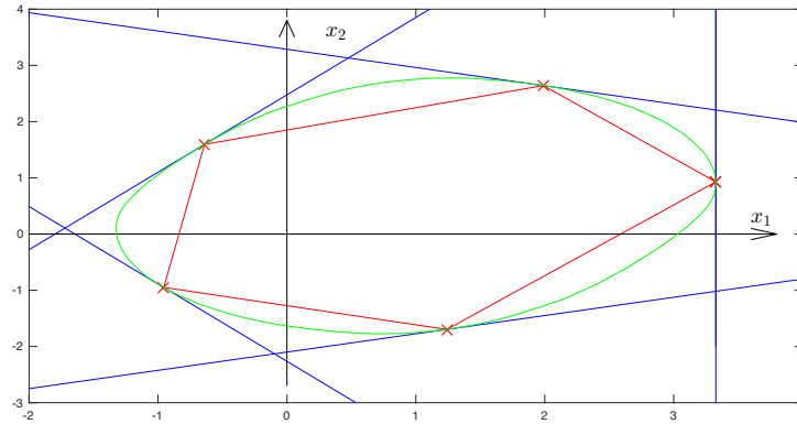
Fig. 2 Approximation of the reachable set.
