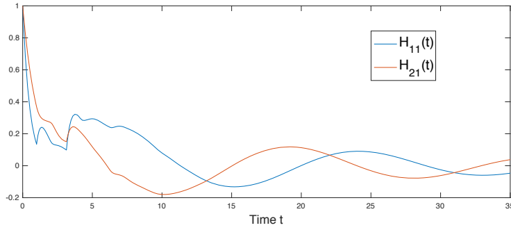
Fig. 1 Graphs of the kernels H_{11}(t) and H_{21}(t) .
