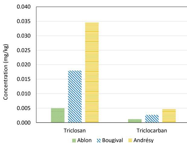
Figure 2. Concentrations of TCS and TCC accumulated in membranes exposed in the Seine river from upstream (Ablon) to downstream (Andrésy)
