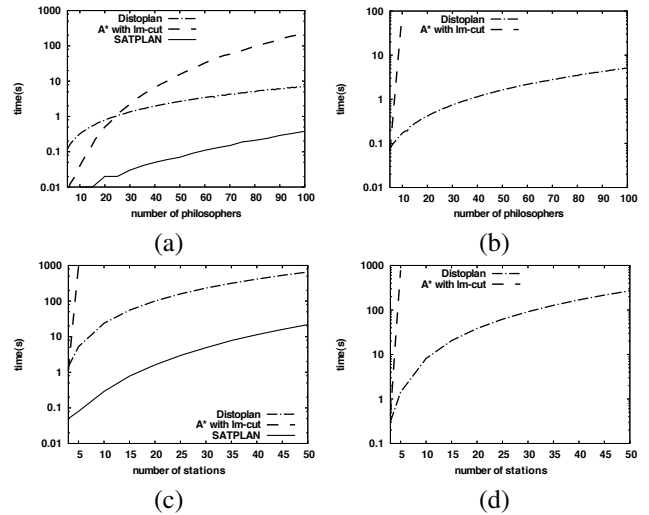
Figure 3: Planner runtimes (logarithmic scale) on the alternative PDDL encodings of Promela domains: (a) Philosophers, deadlockable; (b) Philosophers, deadlock free; (c) Optical-Telegraph, deadlockable; (d) Optical-Telegraph, deadlock free.
