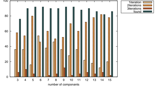
Fig. 3. Experimental results for circles of 3 to 15 automata.
