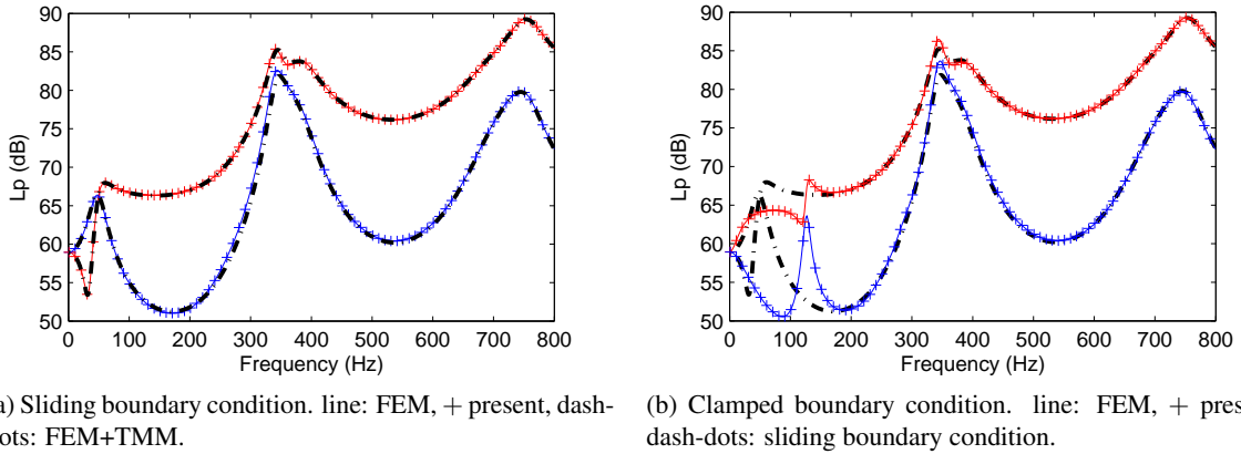
Figure 5: Sound pressure levels in excitation between 1Hz and 800Hz. Red: emission room and blue: reception room.
