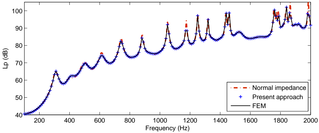
Figure 3: Sound pressure level in the acoustic cavity.
