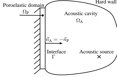
Figure 1: Description of a poroacoustic problem.
