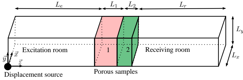
Figure 4: Description and notation for the transmission problem.
