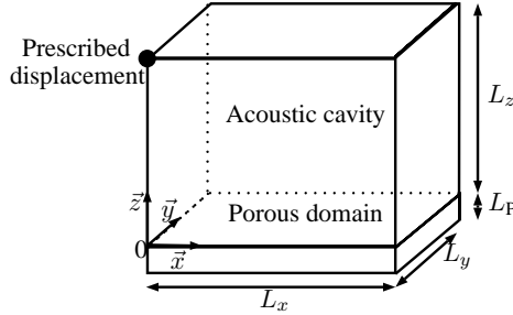
Figure 2: Description and notation for the absorption problem.
