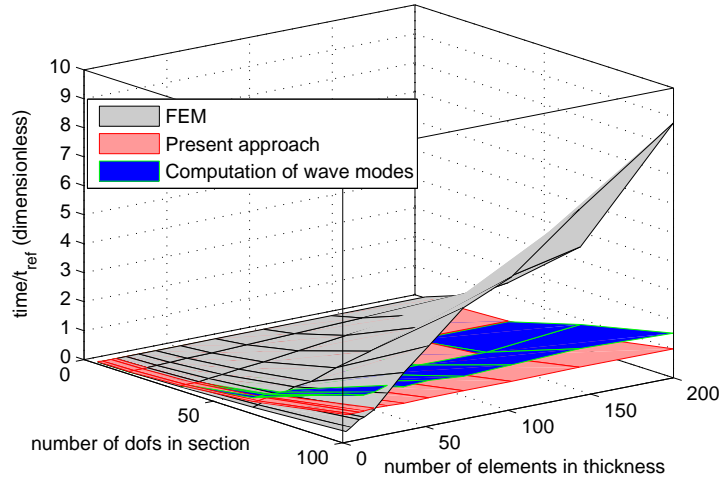
Figure 7: Relative computation times obtained for the absorption problem with 10 acoustic elements along z direction, depending on the number of dofs in the section, the number of elements in thickness and the method.
