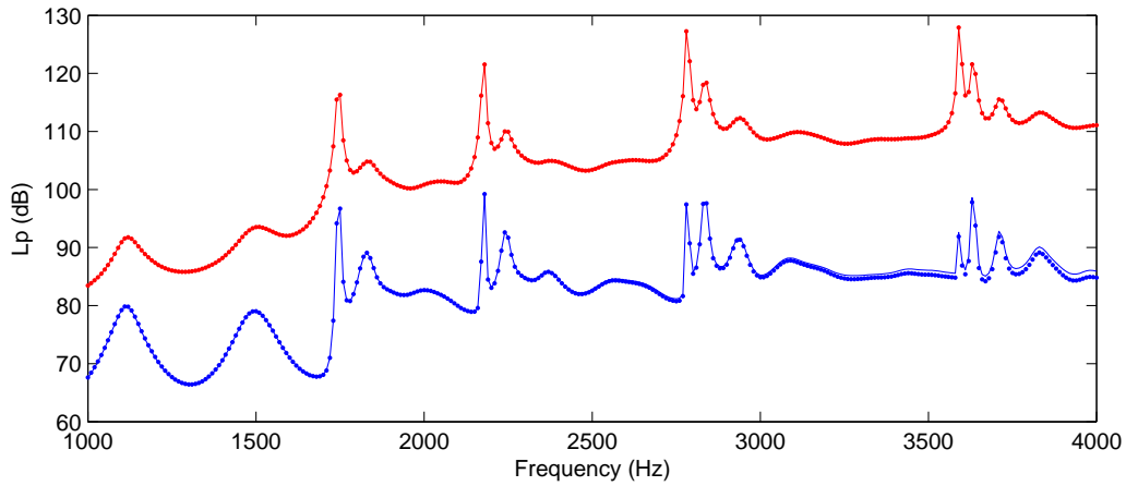
Figure 6: Pressure levels in the higher frequency range. Red: Emission room, blue: reception room. line: FEM, dots: present approach.
