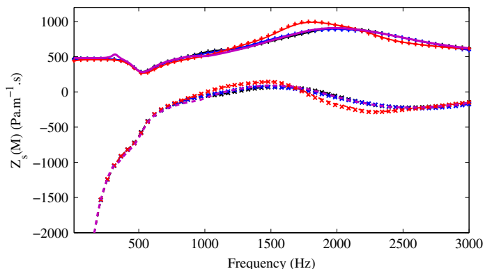
Fig. 11. (Color online) Nodal impedance on observation points. FEM: — real part, - - - imaginary part. WFE: + real part, x imaginary part. M_1 : black, M_2 : blue, M_3 : red. TMM (incidence \theta = 45^\circ ): magenta.
