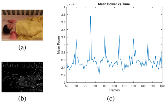
Figure 4: Subtle motion detection for breathing measurement. (a) is the a frame of a video of a baby sleeping, (b) is the masked phase norm and (c) is the obtained signal
