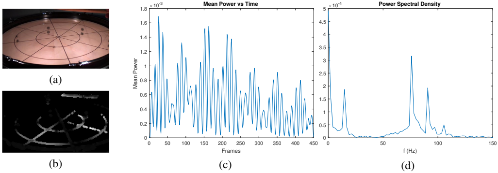
Figure 5: Subtle motion analysis for spectral analysis. (a) is the a frame of a video of a vibrating drum, (b) is the masked phase norm,(c) is the obtained sinusoidal signal and (d) is its magnitude spectrum
