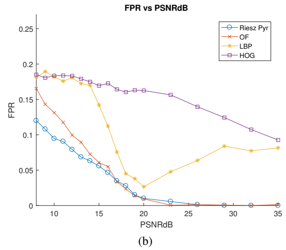
Figure 7: Performance curves of different subtle motion spotting techniques in presence of different levels of Salt and Pepper noise
