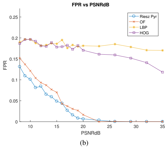
Figure 6: Performance curves of different subtle motion spotting techniques in presence of different levels of Gaussian noise
