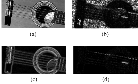
Figure 3: Quaternionic phase masked. (a) is an input video in which the first string of the guitar is subtly oscillating. (b) is the calculated quaternionic phase shift \Delta\phi and (c) is its local amplitude. (d) is the result of masking (b) with (c)
