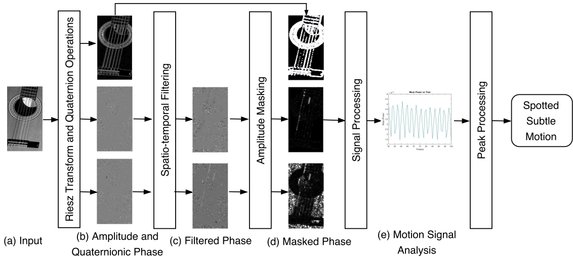
Figure 1: Subtle motion analysis framework. Each frame from an input video (a) is processed with the Riesz Pyramid to obtain the local amplitude and the quaternionic phase (b). We apply an improved spatio-temporal filter to the quaternionic phase (c). Then we use local amplitude to mask relevant areas in the quaternionic phase (d). The phase is processed into a 1-D signal (e) and we detect and classify the resulting peaks to spot the subtle motions.
