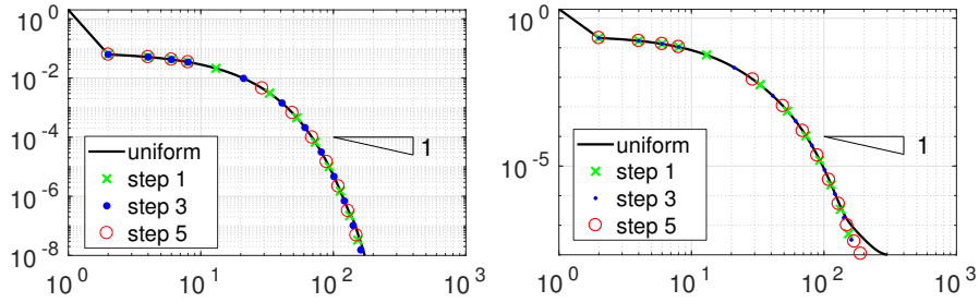
Figure 2: Discrete residual vs. ADMM iteration number for \text{Bi} = 0.3 (left) and \text{Bi} = 0.9 (right) for a fine uniform triangulation with h = 0.0075 and for locally refined meshes at adaptation levels \ell \in \{1, 3, 5\} .
