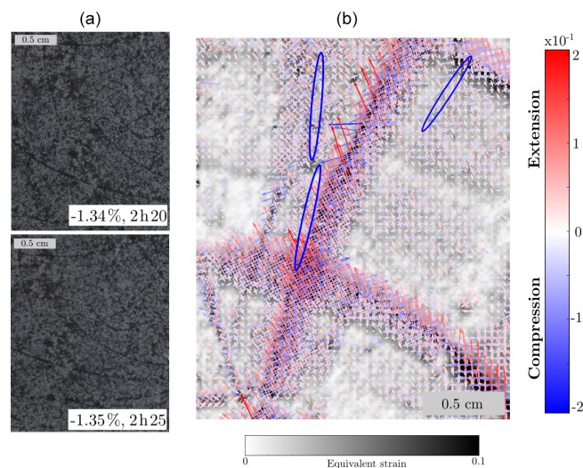
Figure 7. Strain field increment during the 5 min before the apparition of cracks between -1.34 and -1.35\% of macroscopic strain. (a) Pictures of the speckled surface used for the DIC. (b) Principal component of the strain field superimposed on the equivalent strain field ( \varepsilon_{eq} ).
