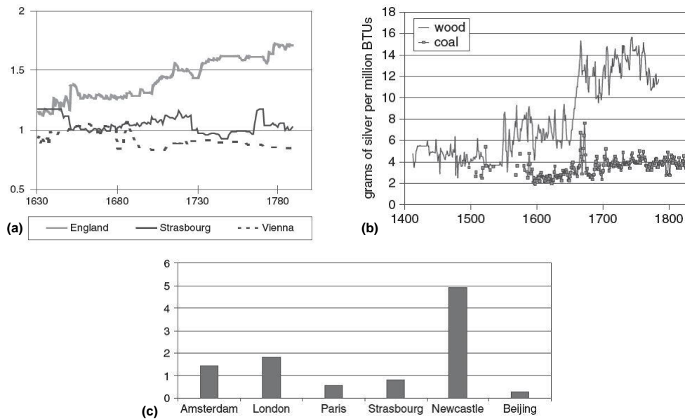
Figure 2: (a) Wage relative to price of capital in three European cities, 1630-1790; (b) Real prices of wood and coal in London, 1400-1825; (c) Wage relative to price of energy in six cities, early 1700s. Source: Allen, 2009 , p.139, 87, and 140 respectively).
