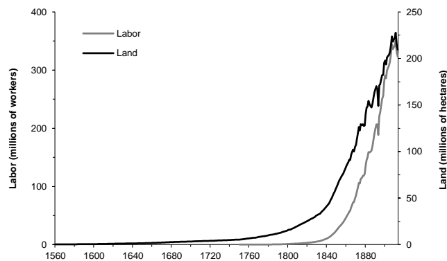
Figure 3: Land (millions of hectares, right vertical axis) and labor (millions of workers, left vertical axis) saved by the use of coal in England and Wales, 1560–1913. Source: Malanima (2016) .
