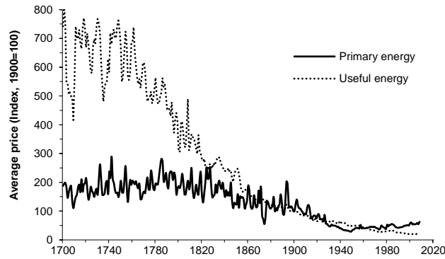
Figure 1: Average prices of primary and useful energies in Great Britain, 1700–2008. Source: Fouquet (2011) .
