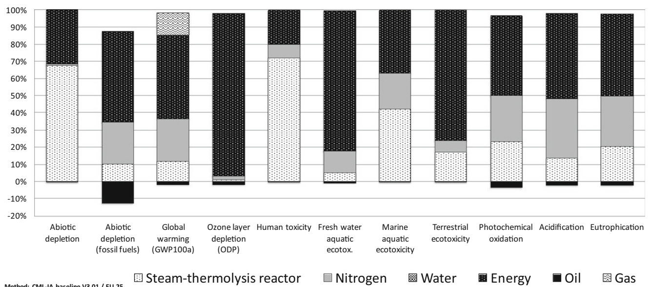
Fig. 7 Impacts associated with the steam thermolysis process—CML-IA baseline
