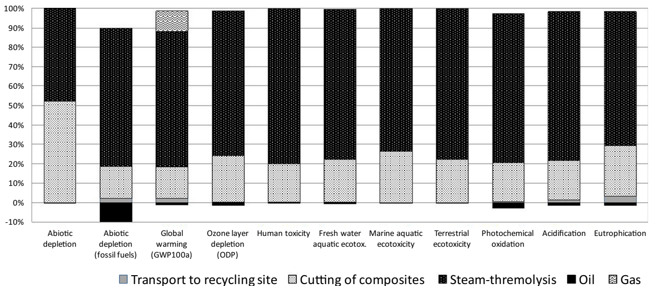
Method: CML-IA baseline V3.01 / EU 25 Fig. 5 Impacts associated with the recycling phase—CML-IA baseline
