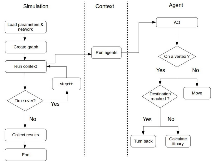
Fig. 1: Steps of a simulation
