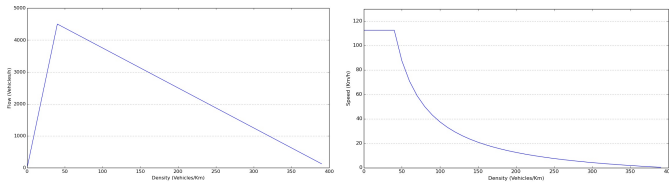
Fig. 2: Fundamental diagram (left) Speed in function of density (right)
