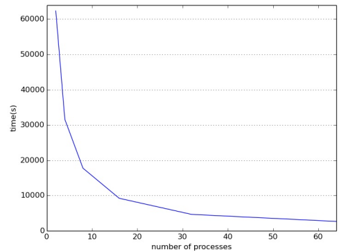
Fig. 11: Execution time in function of the number of processes
