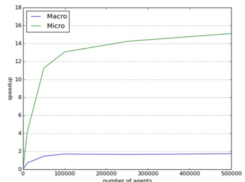
Fig. 8: Speedup for the environment-based distribution
