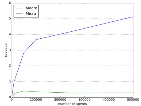
Fig. 7: Speedup for the agent-based distribution
