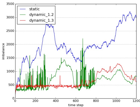
Fig. 9: Load imbalance
