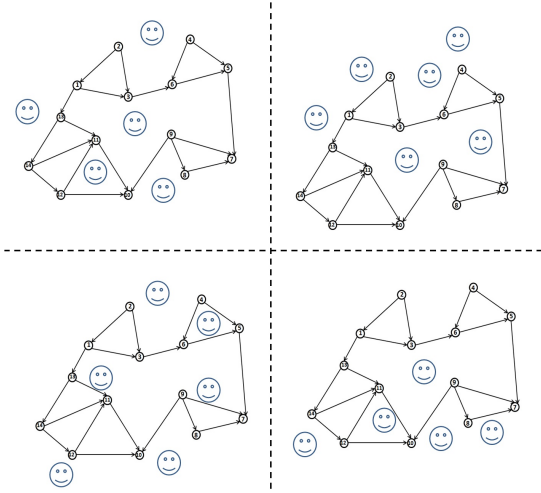
Fig. 4: Agents distribution
