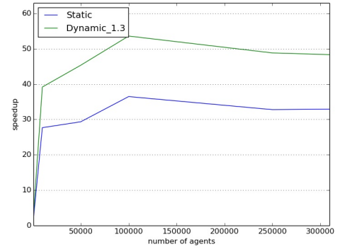
Fig. 10: Speedup for the different methods
