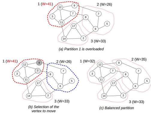
Fig. 6: Diffusive load balancing
