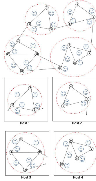
Fig. 5: Environment distribution
