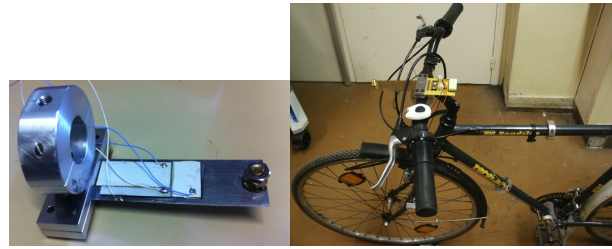
Fig. 8. Harvester with piezoelectric layer and tip mass.
