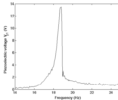
Fig. 17. Experimental frequency response result: acceleration 2 \text{ m/s}^2 .
