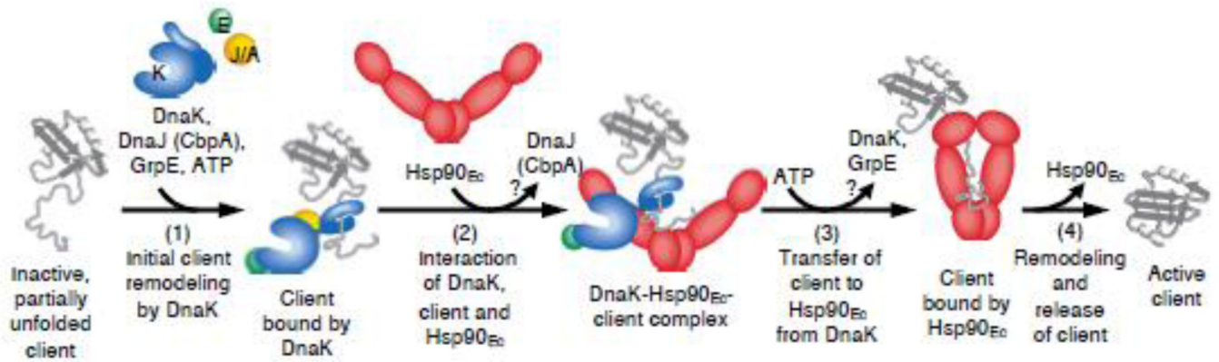
Fig. 7. Working model for the mechanism of action of the DnaK system in collaboration with Hsp90 Ec . First, the client protein is bound by DnaK for initial ATP-dependent remodeling, a process that requires DnaJ/CbpA and GrpE (step 1). Next, DnaK, through a direct interaction of the DnaK NBD with the Hsp90 Ec middle domain, recruits Hsp90 Ec to the client, which further stabilizes the interaction between DnaK and Hsp90 Ec (step 2). DnaJ/CbpA may be released at this time. Binding and hydrolysis of ATP by Hsp90 Ec triggers conformational changes in the chaperone that lead to client transfer and stabilization of client binding to Hsp90 Ec (step 3). DnaK and GrpE may be released at this step. Hsp90 Ec promotes further client remodeling and releases the active native client (step 4). Client proteins that do not attain the active conformation may reenter the chaperone cycle.
