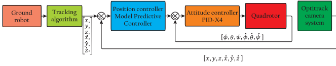
Fig. 5. Final control architecture
