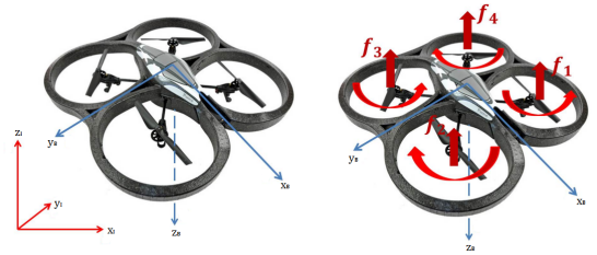
Fig. 1. Inertial and body frames
