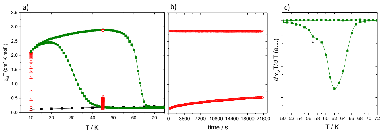
Figure 6: (a) Light-Induced Thermal Hysteresis recorded at 0.3 \text{ K min}^{-1} under a permanent irradiation at 532 \text{ nm} ( 5 \text{ mW cm}^{-2} ) with photostationary points ( \Delta and \nabla ) at 10 \text{ K} and 45 \text{ K} . (b) Temporal view of the photostationary points. (c) Derivative of \chi_M T product evidencing the presence of an inflexion at 58 \text{ K} (arrow).
