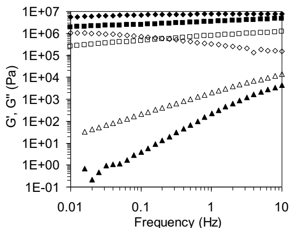
Figure 5. Rheological properties of PDMS(30)-g-BuP (◆, ◇), PDMS(37)-g-NMeP (■, □), and PDMS(30)-g-Ph (▲, △) at 30^\circ\text{C} . Elastic modulus G' (full symbols), loss modulus G'' (hollow symbols).
