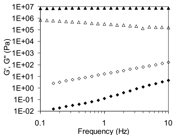
Figure 4. Rheological properties of bis-urea grafted PDMS(30)-g-BuP (▲, △) and its amino functional precursor (◆, ◇) at 30^\circ\text{C} . Elastic modulus G' (full symbols), loss modulus G'' (hollow symbols).
