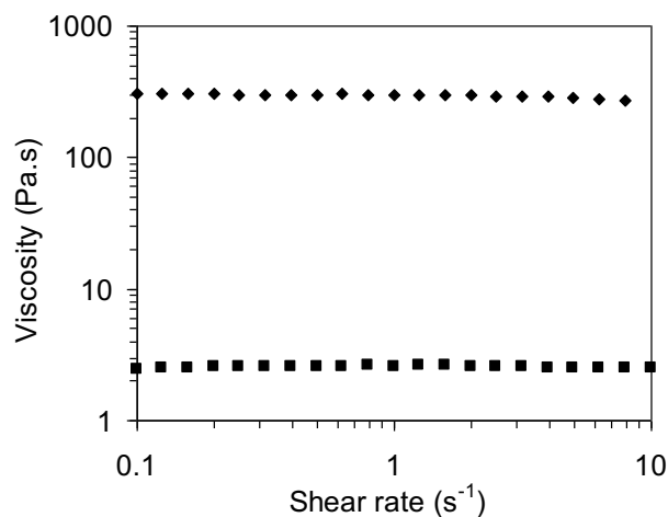
Figure 7. Viscosity of PDMS(30)-g-Ph ( \blacklozenge ) and its amino-functional precursor ( \blacksquare ) at 30°C.
