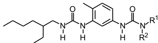
BuP/EH
