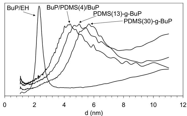
Figure 2. Small angle X-ray scattering curves obtained for three bis-urea functional PDMS (Scheme 1 and Tables 1 and 2) and a model bis-urea (Scheme 2) at 25°C.
