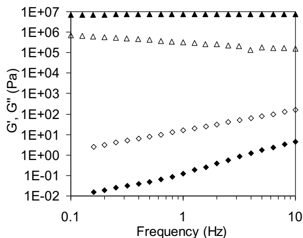
Figure 4. Rheological properties of bis-urea grafted PDMS(30)-g-BuP ( \blacktriangle , \triangle ) and its amino functional precursor ( \blacklozenge , \lozenge ) at 30^\circ\text{C} . Elastic modulus G' (full symbols), loss modulus G'' (hollow symbols).
