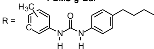
PDMS-g-BuP
