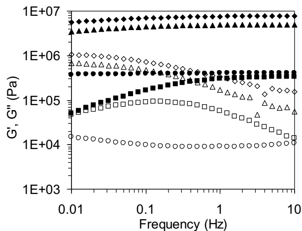
Figure 6. Rheological properties of PDMS(30)-g-BuP ( \blacklozenge , \diamond ), PDMS(13)-g-BuP ( \blacktriangle , \triangle ), BuP/PDMS(29)/BuP ( \bullet , \circ ), and PDMS(10)-g-BuP ( \blacksquare , \square ) at 30°C. Elastic modulus G' (full symbols), loss modulus G'' (hollow symbols).
