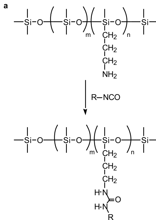
PDMS-g-BuP
