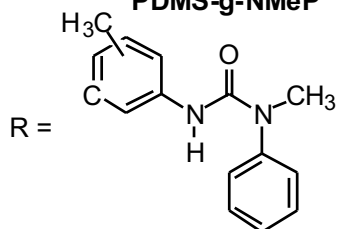
PDMS-g-NMeP
